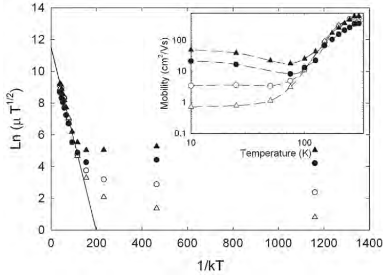
Figure 139: Temperature dependence of the mobility for specimens I (○), II (△), III (●), and VI (▲). Lines are a guide for the eye only. Plotting the logarithm of \mu_{\text{eff}} = \mu_o (1/T)^{1/2} \exp(-E_B/kT) and fitting the high temperature data yields an energy barrier of 60 meV for all specimens.
