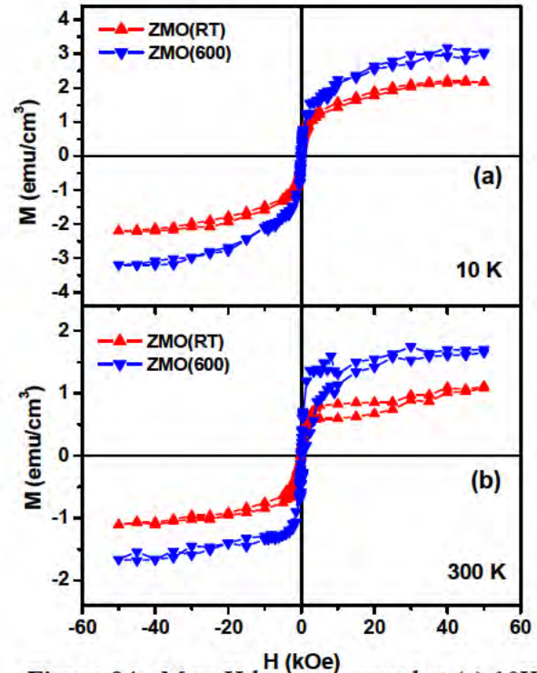
Figure 94: M vs H loops measured at (a) 10K and (b) 300K for (\text{Zn}_{0.98}\text{Mn}_{0.02})\text{O} films deposited on c -cut sapphire substrates at RT and 600 °C with a constant pO_2 of 10mT named as ZMO(RT) and ZMO(600) respectively.
