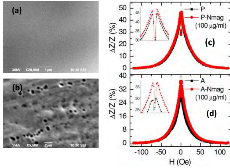
Figure 49: SEM images of plain (a) and Nitric acid \sim 4 vol -%) treated (b) ribbons, and corresponding GMI profiles (c – d) with and with Nanomag-D bead suspension (5 \mu l).
