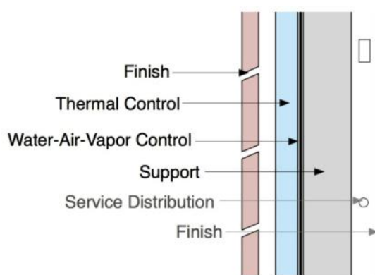
Figure 3-2. Idealized enclosure with service distribution and finishes.
