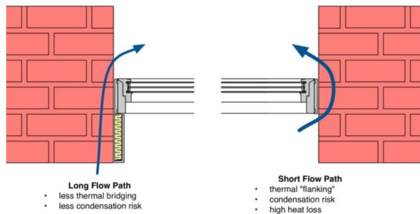
Figure 4-10. Thermal flanking around a new high performance window in a thick solid masonry wall.
