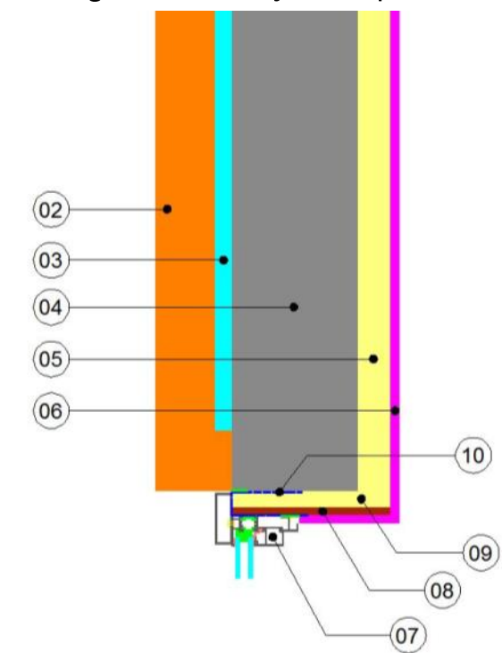
Figure 7-6. Window jamb – improved.
