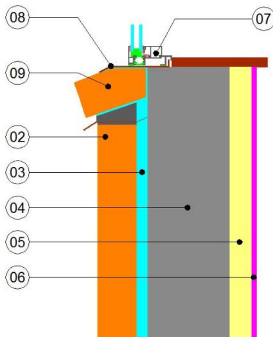
Figure 7-9. Window sill – corrected.
