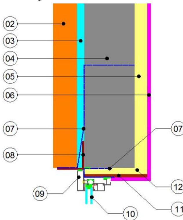
Figure 7-8. Window head – corrected.
