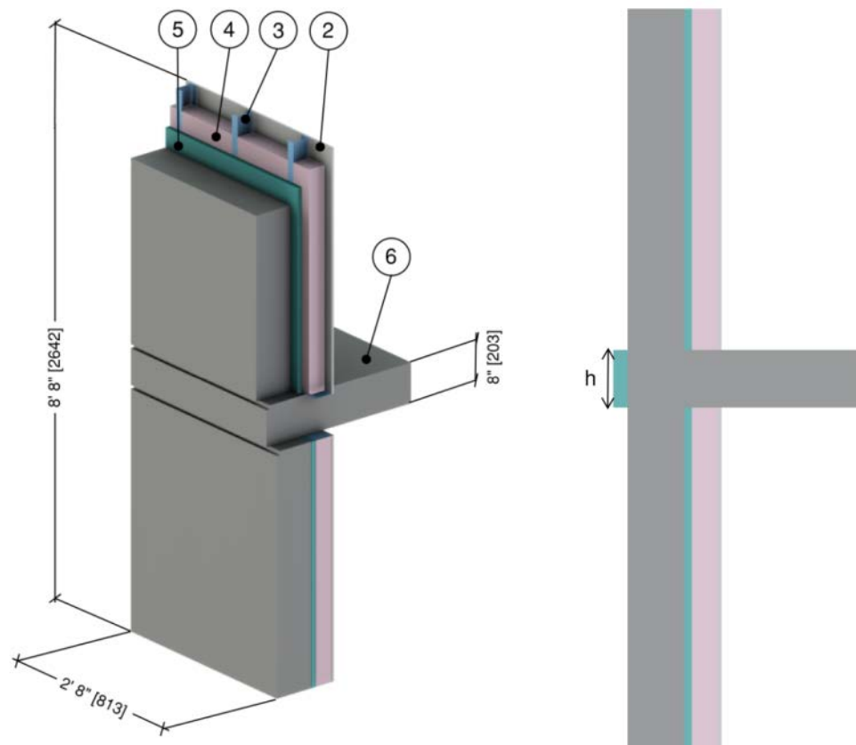
Figure 7-2. Suspended slab.
