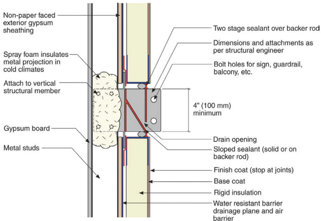
Figure 4-9. Insulation on the inside of structural connection penetrating insulation to control cold weather condensation.
