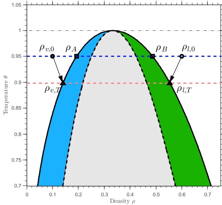
Figure 6: Illustration of the thermal bubble dynamics. \rho_{v,0} and \rho_{l,0} are the initial vapor and liquid densities; \rho_A and \rho_B are the Maxwell state at the initial temperature; \rho_{v,T} and \rho_{l,T} are the vapor and liquid densities at time T = 10.0 .
