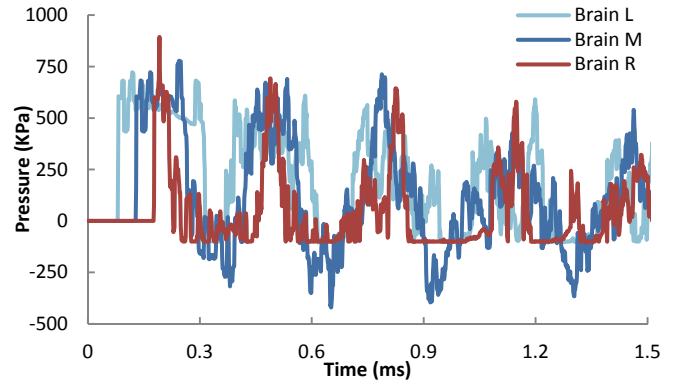
Figure 9 The time histories of pressure (positive in compression) in the brain
