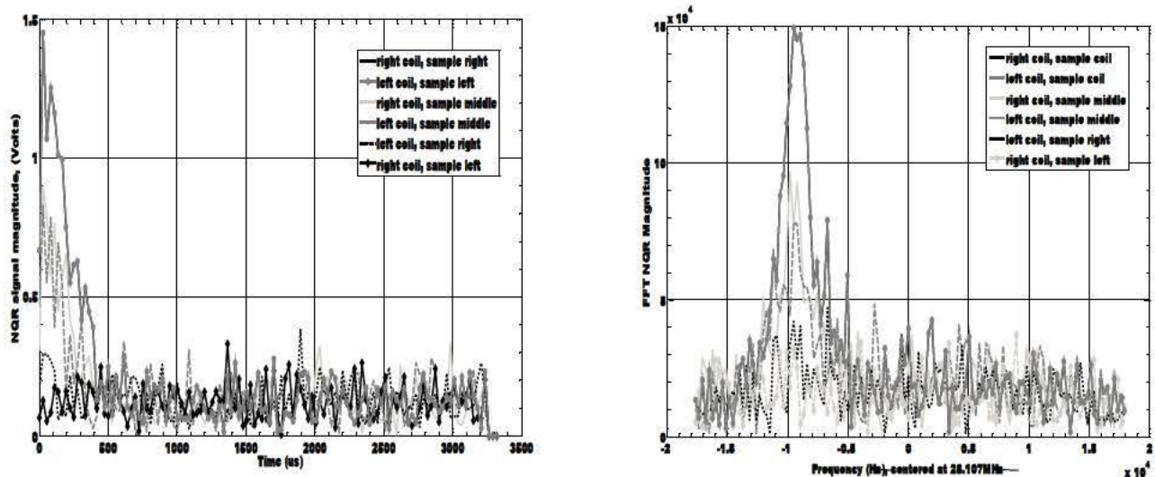
Fig.7, (left) time domain of the magnitude of the NQR signal from the different configurations, and (right) the FFT of NQR signal from different configurations with the center frequency being 28.1MHz
