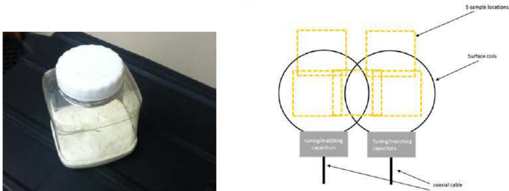
Fig.5, potassium chlorate in container outside of the RF shield (left), and diagram of both left and right coil configurations (right)
