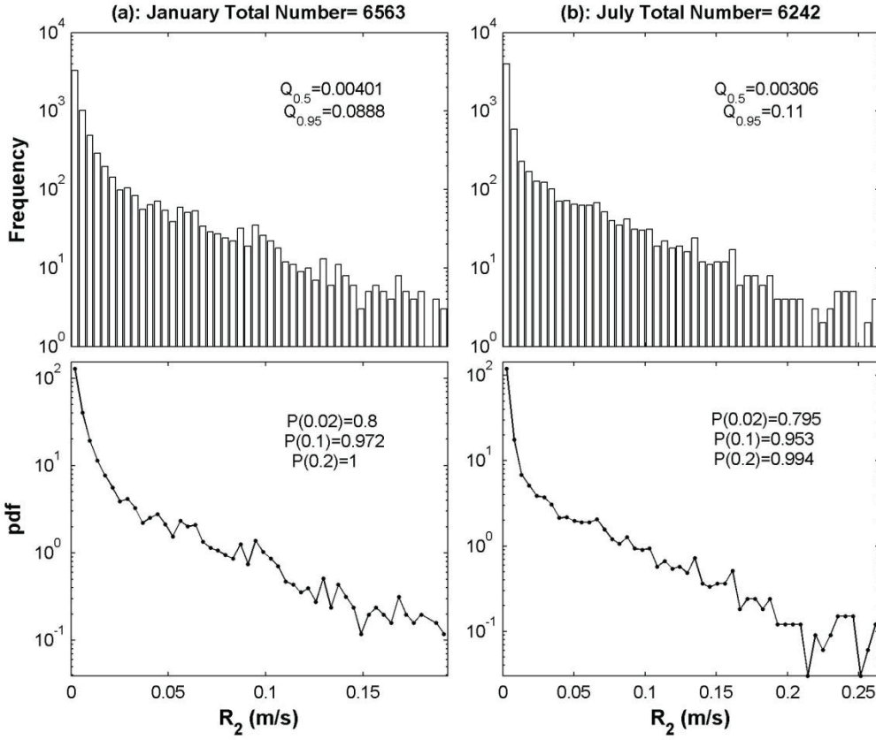
Fig. 17. Histogram and probability density function of R_2 ( \text{m s}^{-1} ) inside the mixed layer with wind-dependent and depth-independent eddy viscosity \hat{K}(0) : (a), January, and (b) July.
