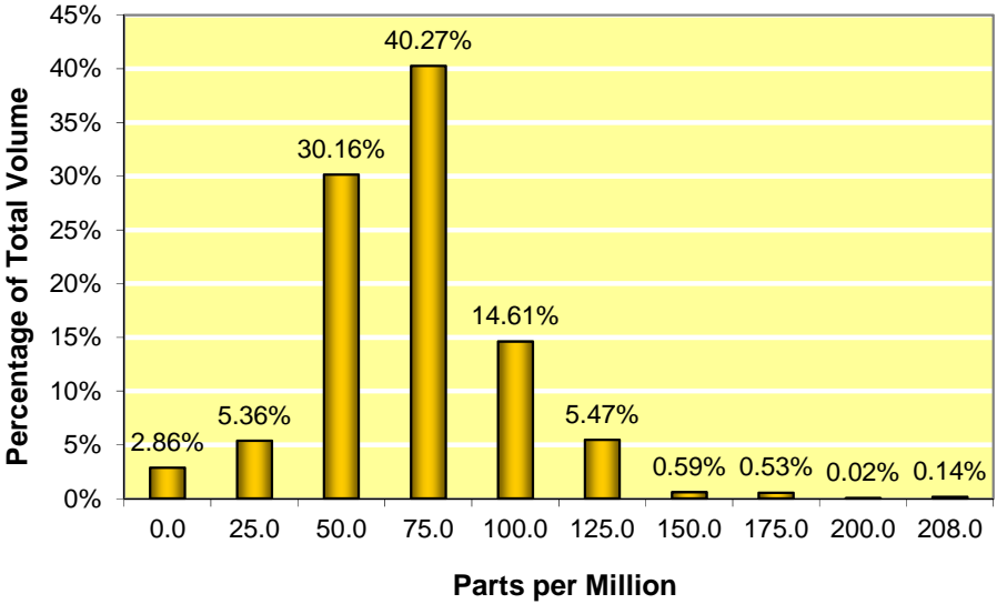
Figure 4-39: Water Content, January–June 2012
