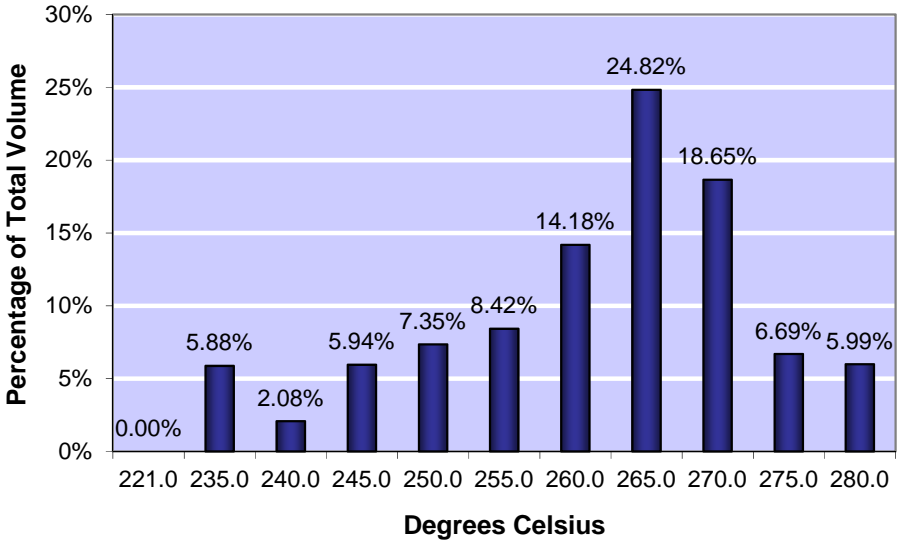
Figure 6-13: Distillation Final Boiling Point (°C), maximum 300.0
