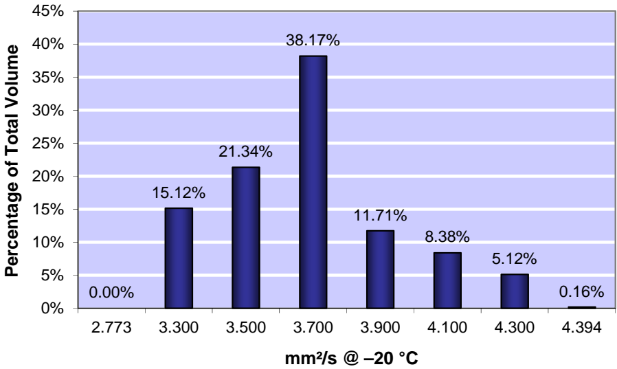
Figure 6-24: Viscosity (mm 2 /s @ -20 °C), maximum 8.0
