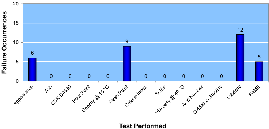
Figure 8-19: MGO In-Line Sampling Program, Characteristic Failure Occurrences, ISO-8217, Marine Gas Oil, Grade DMA Requirements, CY 2012
