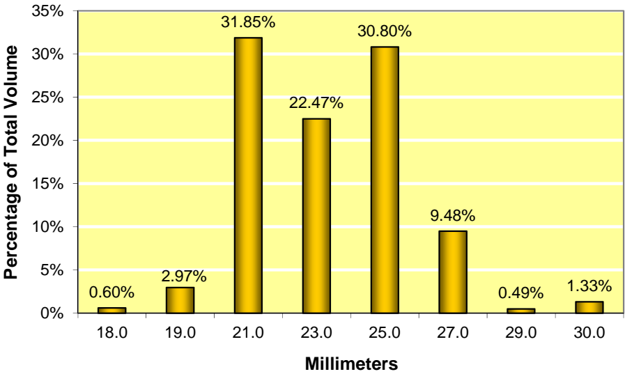
Figure 4-27: Smoke Point (mm), minimum 25.0
