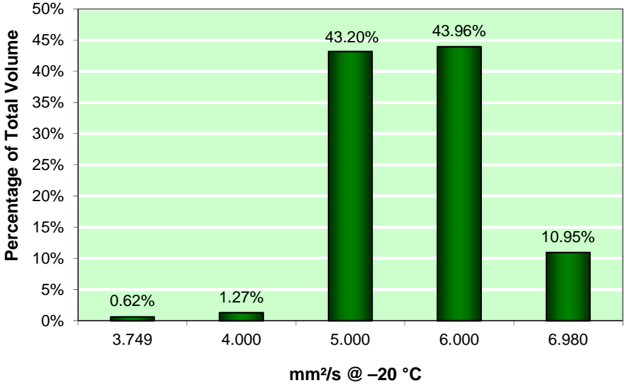
Figure 5-23: Viscosity (mm 2 /s @ -20 °C), maximum 8.5
