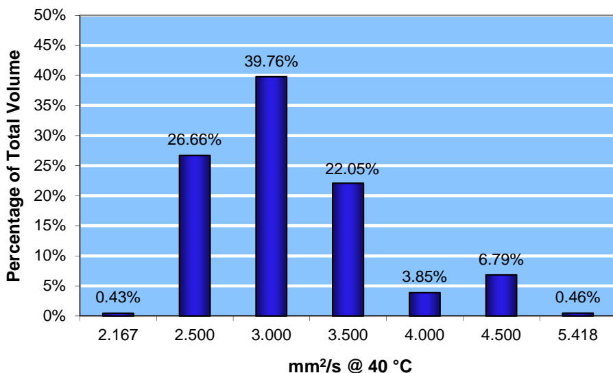
Figure 8-5: Kinematic Viscosity (mm 2 /s @ 40 °C), minimum 2.000, maximum 6.000
