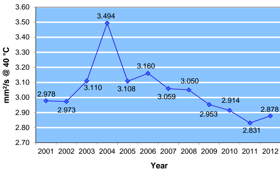
Figure 8-6: Kinematic Viscosity (mm 2 /s @ 40 °C), 12-Year Trend, minimum 2.000, maximum 6.000
