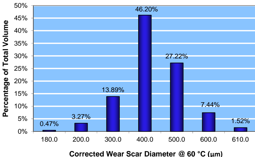
Figure 8-15: Lubricity, corrected wear scar diameter @ 60 °C (µm), maximum 520
