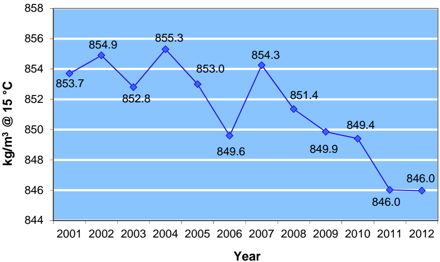
Figure 8-8: Density (kg/m³ @ 15 °C), 12-Year Trend, maximum 890
