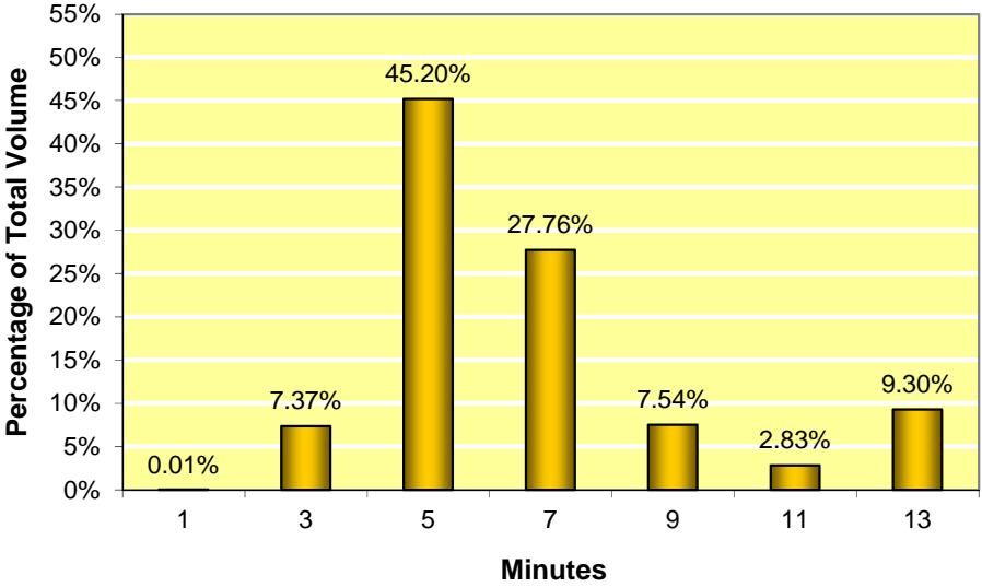
Figure 4-35: Filtration Time (minutes), maximum 15
