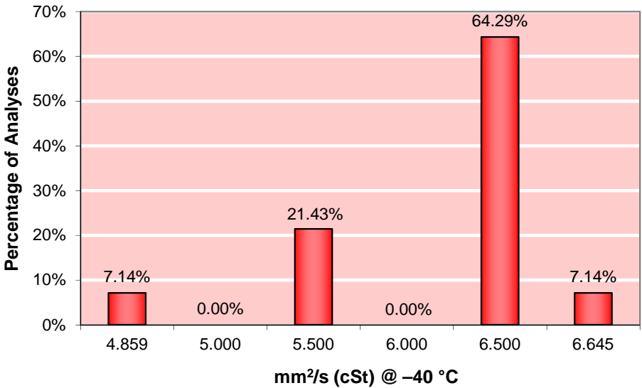
Figure 9-8: Viscosity (mm 2 /s [cSt] @ -40 °C), Report
