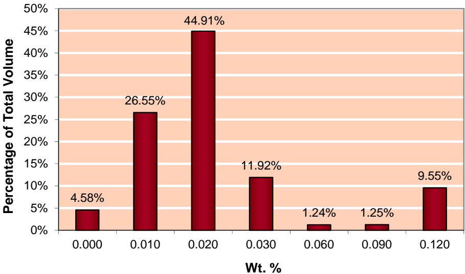
Carbon Residue on 10% Bottoms—2012 (Methods ASTM D-189 and D-4530)
