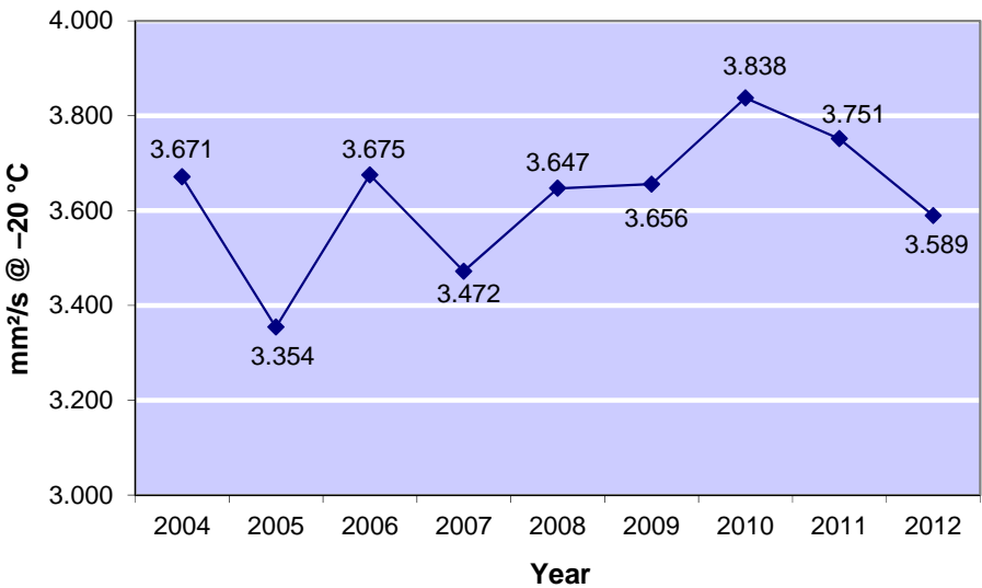
Figure 6-25: Viscosity (mm 2 /s @ -20 °C), 9-Year Trend, maximum 8.0
