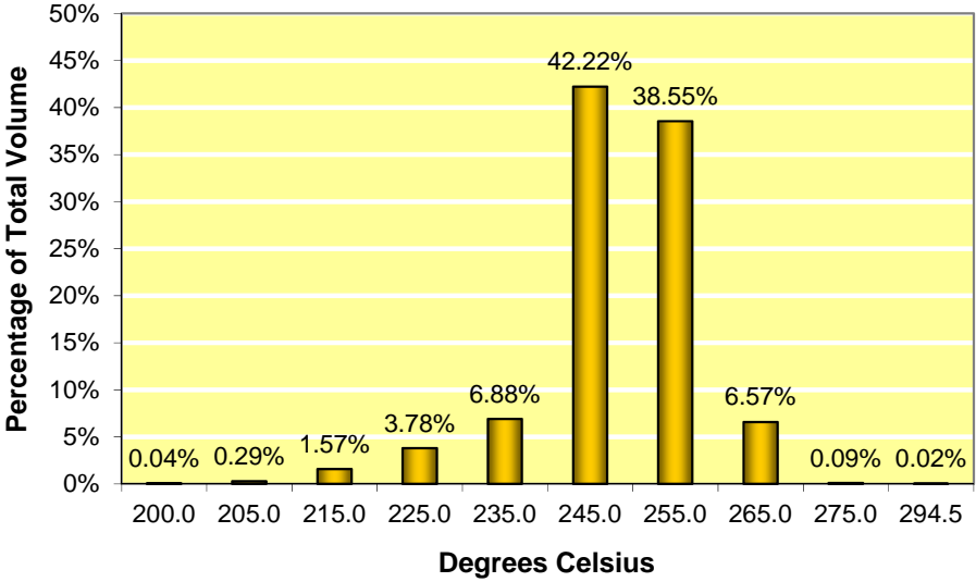
Figure 4-11: Distillation 90% Recovered (°C), Report
