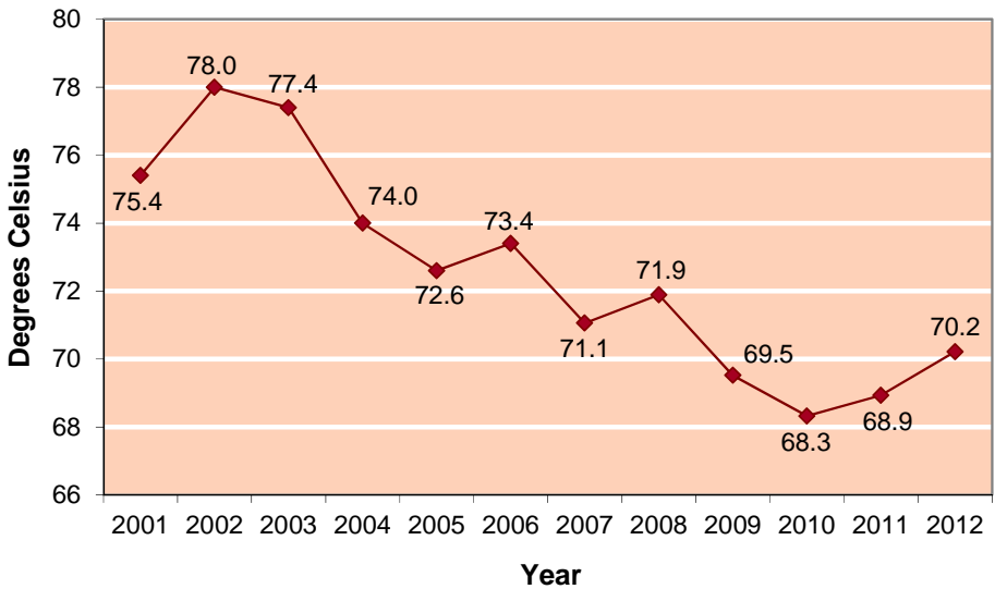
Figure 7-11: Flash Point (°C), 12-Year Trend, minimum 60
