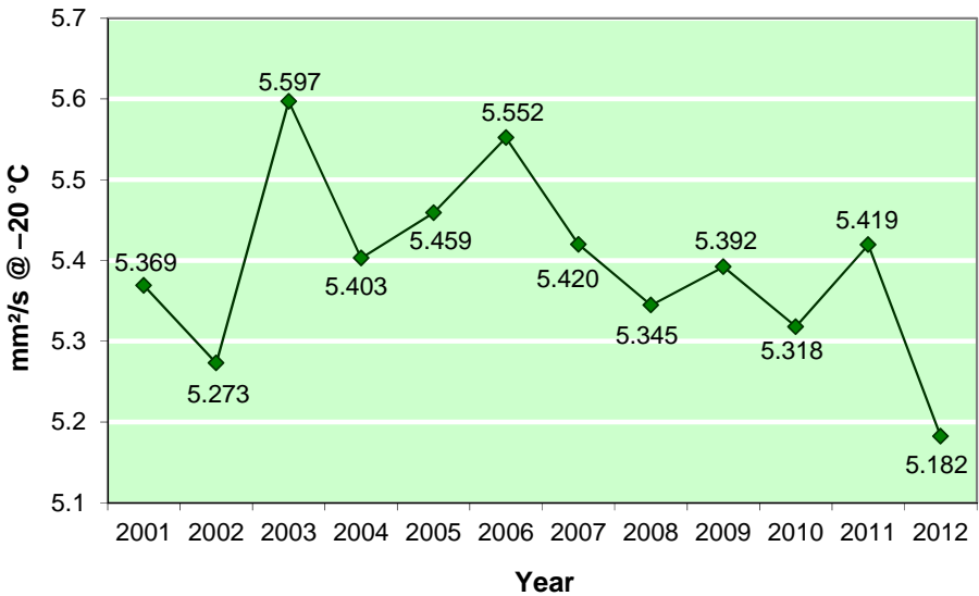
Figure 5-24: Viscosity (mm 2 /s @ -20 °C), 12-Year Trend, maximum 8.5
