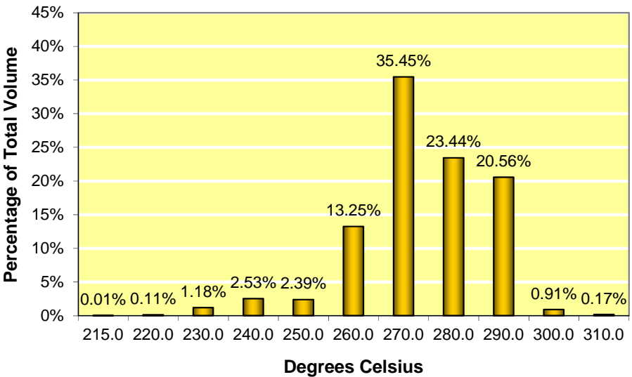
Figure 4-12: Distillation Final Boiling Point (°C), maximum 300
