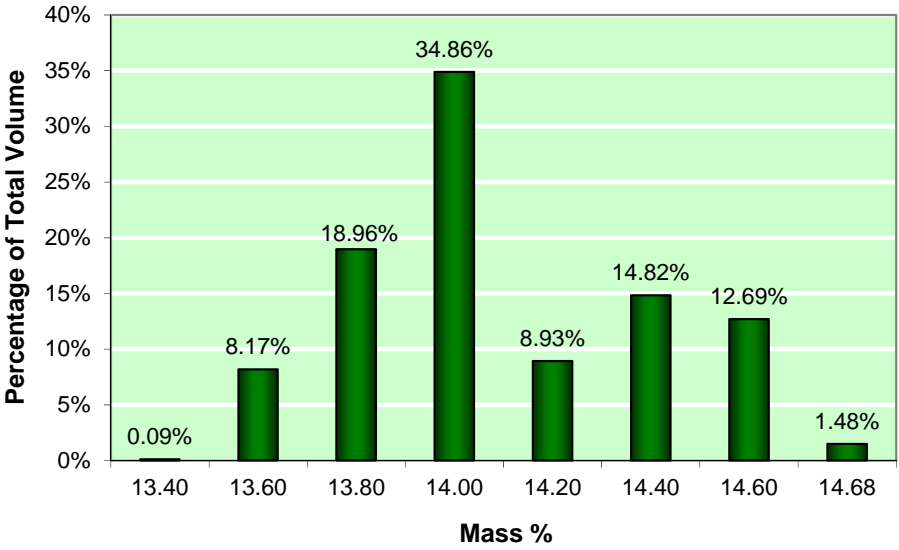
Figure 5-27: Hydrogen Content (mass %), minimum 13.4
