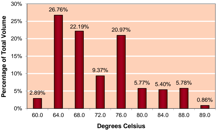
Figure 7-10: Flash Point (°C), minimum 60
