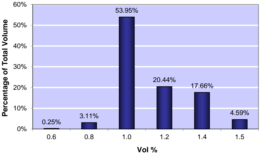
Figure 6-15: Distillation Residue (vol %), maximum 1.5
