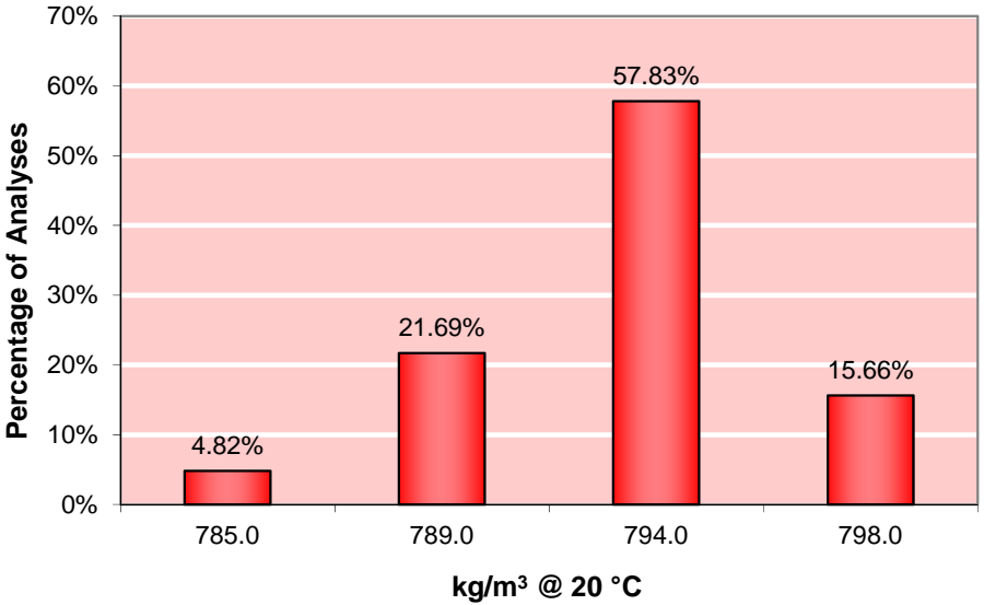
Figure 9-1: Density (kg/m 3 @ 20 °C), minimum 775
