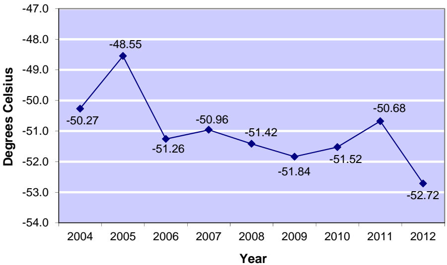
Figure 6-23: Freezing Point (°C), 9-Year Trend, maximum -47
