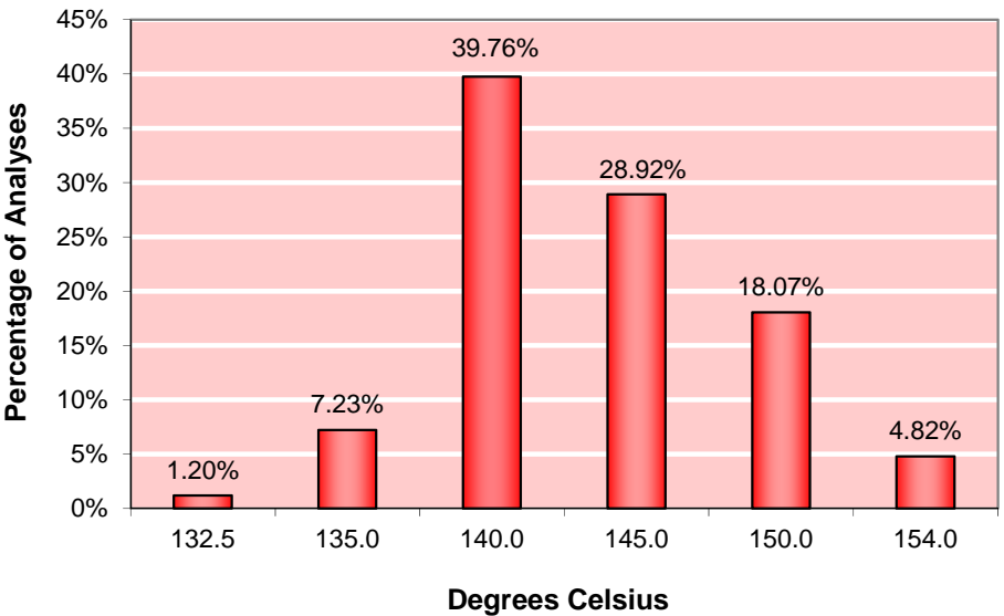
Figure 9-2: Fractional Composition (Distillation), Temperature at Start (Initial Boiling Point) (°C), maximum 150
