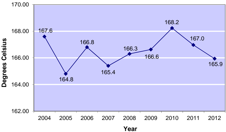
Figure 6-10: Distillation 10% Recovered (°C), 9-Year Trend, maximum 205.0
