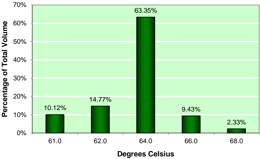
Figure 5-17: Flash Point (°C), minimum 60
