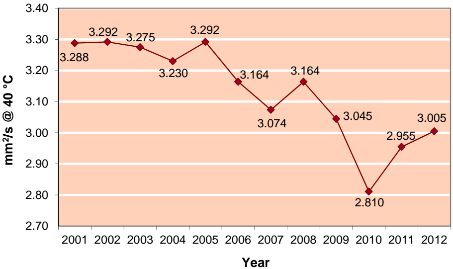
Figure 7-15: Viscosity (mm 2 /s @ 40 °C), 12-Year Trend, minimum 1.7, maximum 4.3
