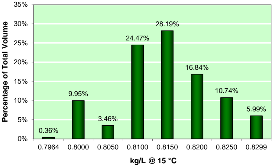
Figure 5-19: Density (kg/L @ 15 °C), minimum 0.788, maximum 0.845
