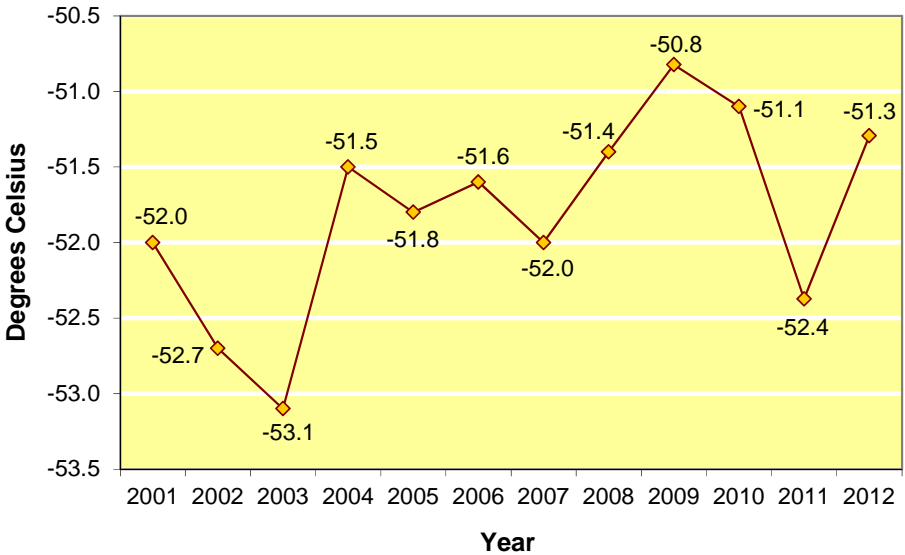
Figure 4-20: Freezing Point (°C), 12-Year Trend, maximum -47
