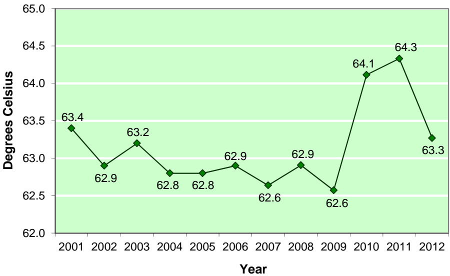
Figure 5-18: Flash Point (°C), 12-Year Trend, minimum 60
