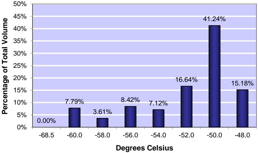
Figure 6-22: Freezing Point (°C), maximum -47
