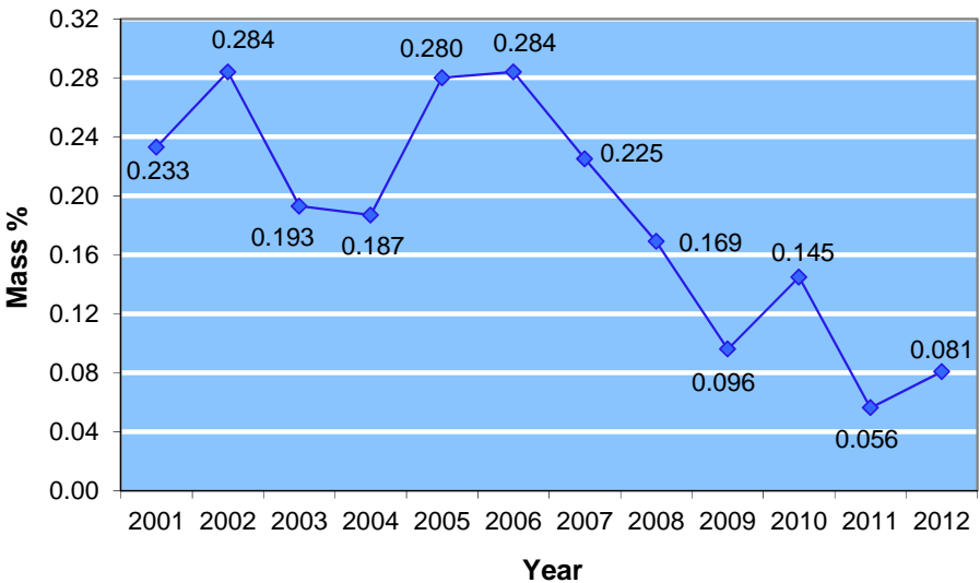
Figure 8-12: Sulfur (mass %), 12-Year Trend, maximum 1.0
