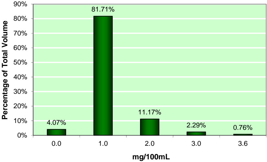
Figure 5-31: Existent Gum (mg/100 mL), maximum 7.0
