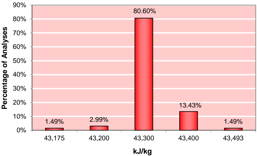
Figure 9-10: Estimate of Heat Value (kJ/kg), minimum 42,900
