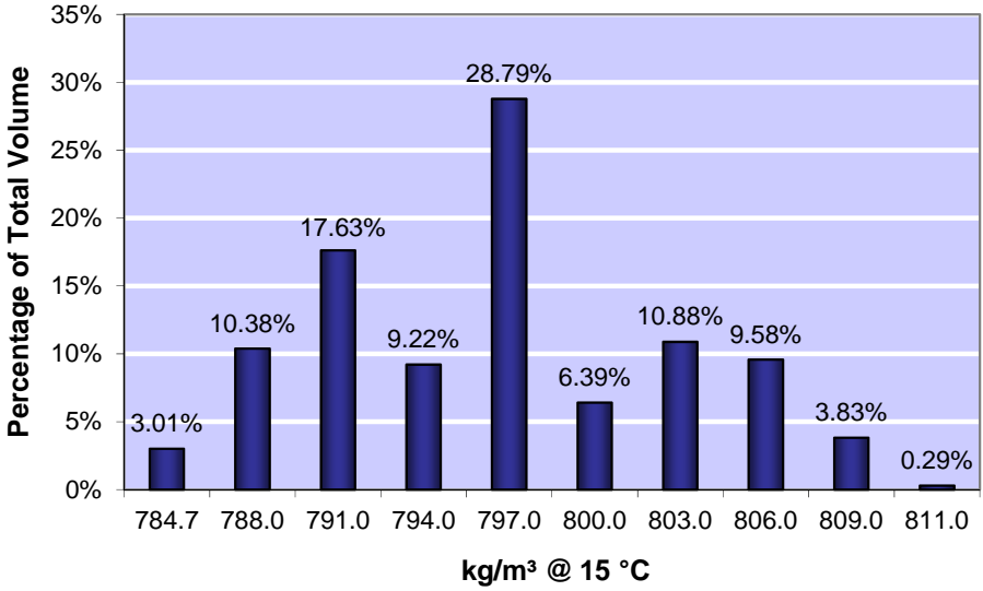
Figure 6-20: Density (kg/m 3 @ 15 °C), minimum 775, maximum 840
