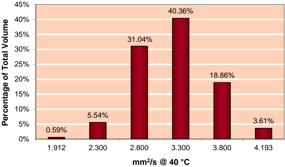
Figure 7-14: Viscosity (mm 2 /s @ 40 °C), minimum 1.7, maximum 4.3
