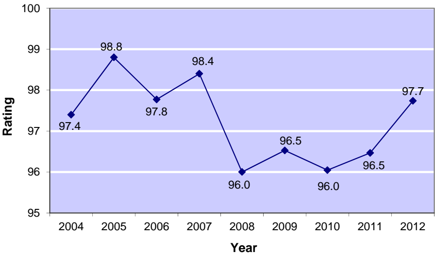
Figure 6-33: Water Separation Index (rating), 9-Year Trend, minimum 70
