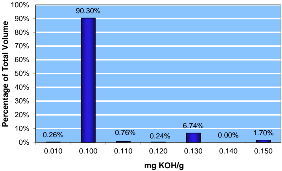
Figure 8-13: Acid Number (mg KOH/g), maximum 0.5
