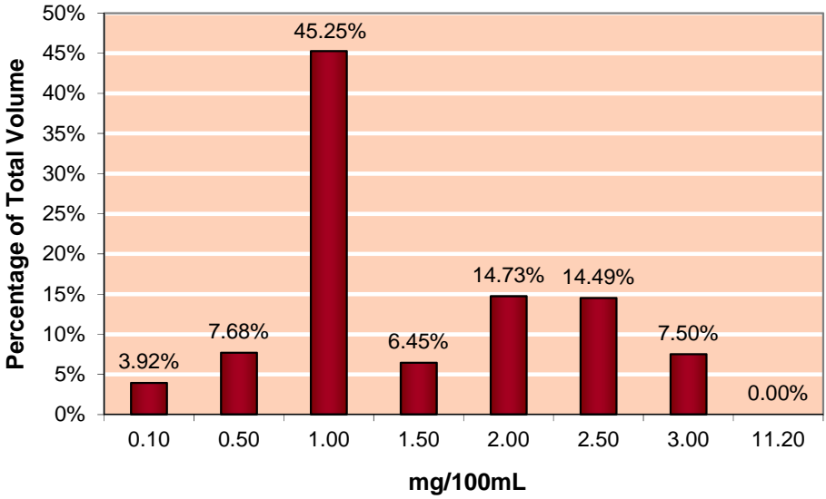
Figure 7-29: Storage Stability: D-5304 (mg/100 mL), maximum 3.0
