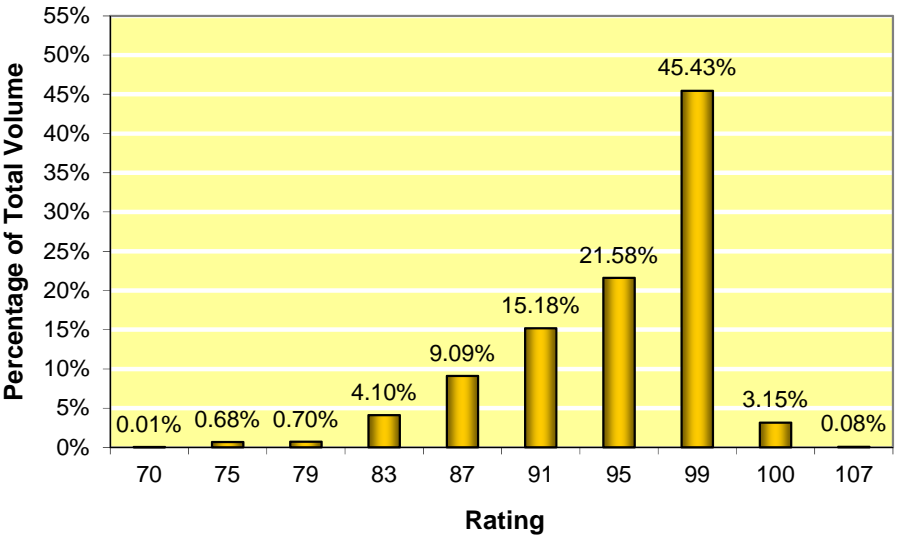
Figure 4-36: Water Separation Index (rating), minimum 70
