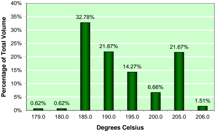
Figure 5-11: Distillation 20% Recovered (°C), Report
