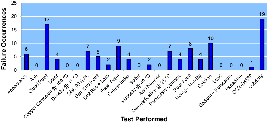
Figure 8-18: MGO In-Line Sampling Program, Characteristic Failure Occurrences, MIL-DTL-16884 Requirements, CY 2012
