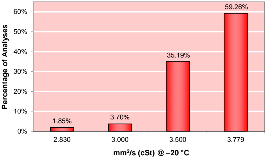
Figure 9-9: Viscosity (mm 2 /s [cSt] @ -20 °C), maximum 8.0
