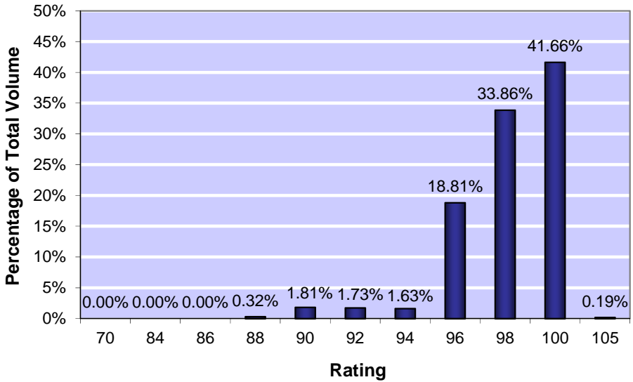
Figure 6-32: Water Separation Index (rating), minimum 70
