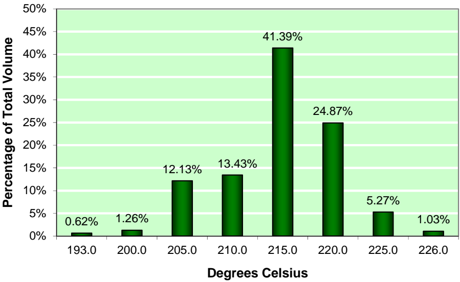
Figure 5-12: Distillation 50% Recovered (°C), Report
