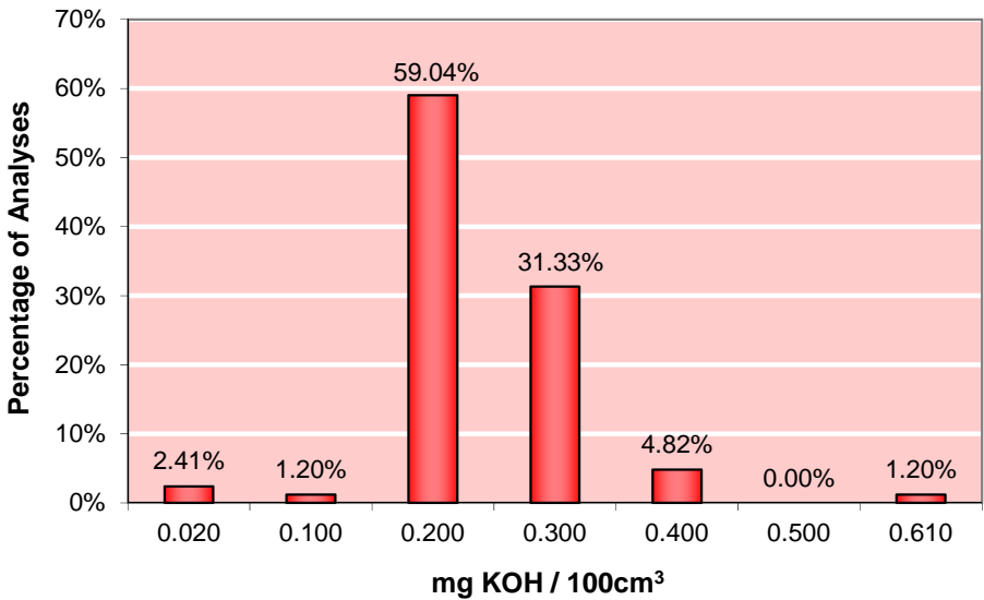
Figure 9-12: Acidity (mg KOH/100cm 3 ), maximum 0.7
