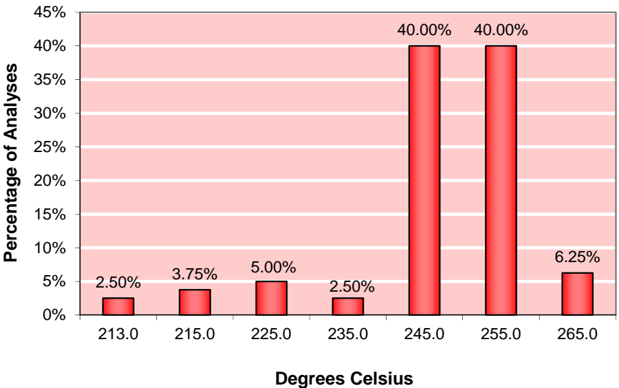
Figure 9-6: Fractional Composition (Distillation), 98% Recovered (°C), maximum 250
