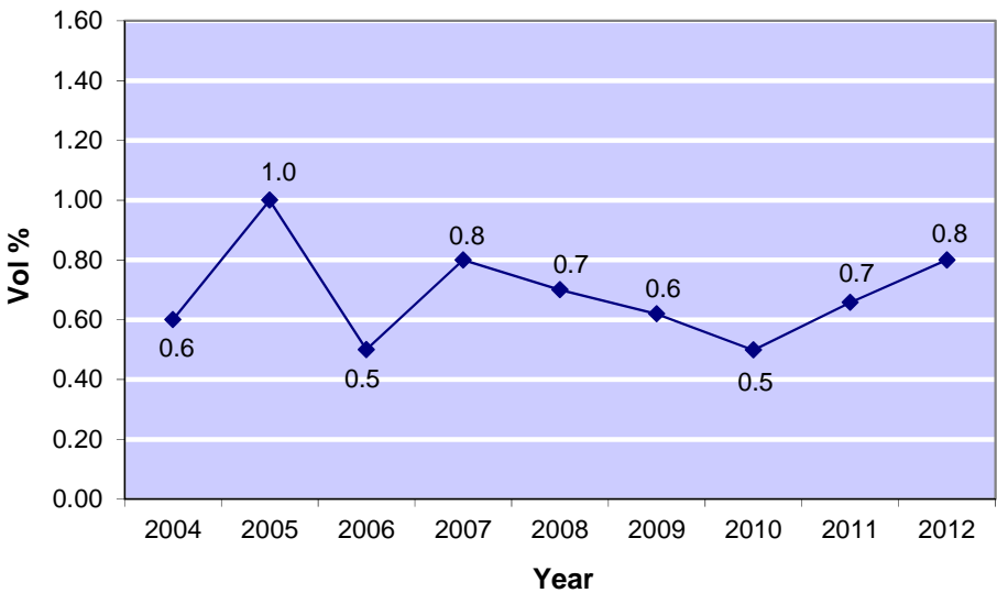
Figure 6-17: Distillation Loss (vol %), 9-Year Trend, maximum 1.5
