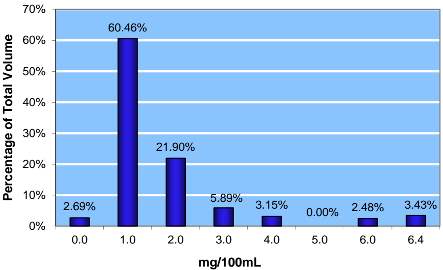
Figure 8-14: Oxidation Stability (mg/100 mL), maximum 25
