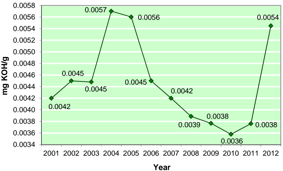
Figure 5-2: Total Acid Number (mg KOH/g), 12-Year Trend, maximum 0.015
