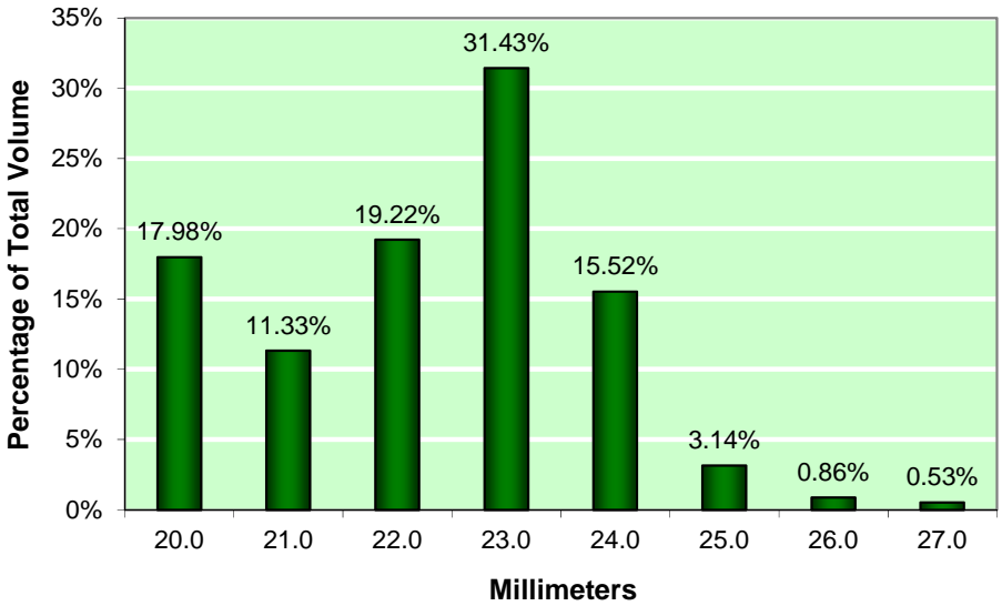
Figure 5-29: Smoke Point (mm), minimum 19.0
