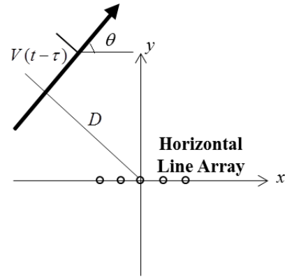
Fig. 2. Parameters that define a constant velocity trajectory.
