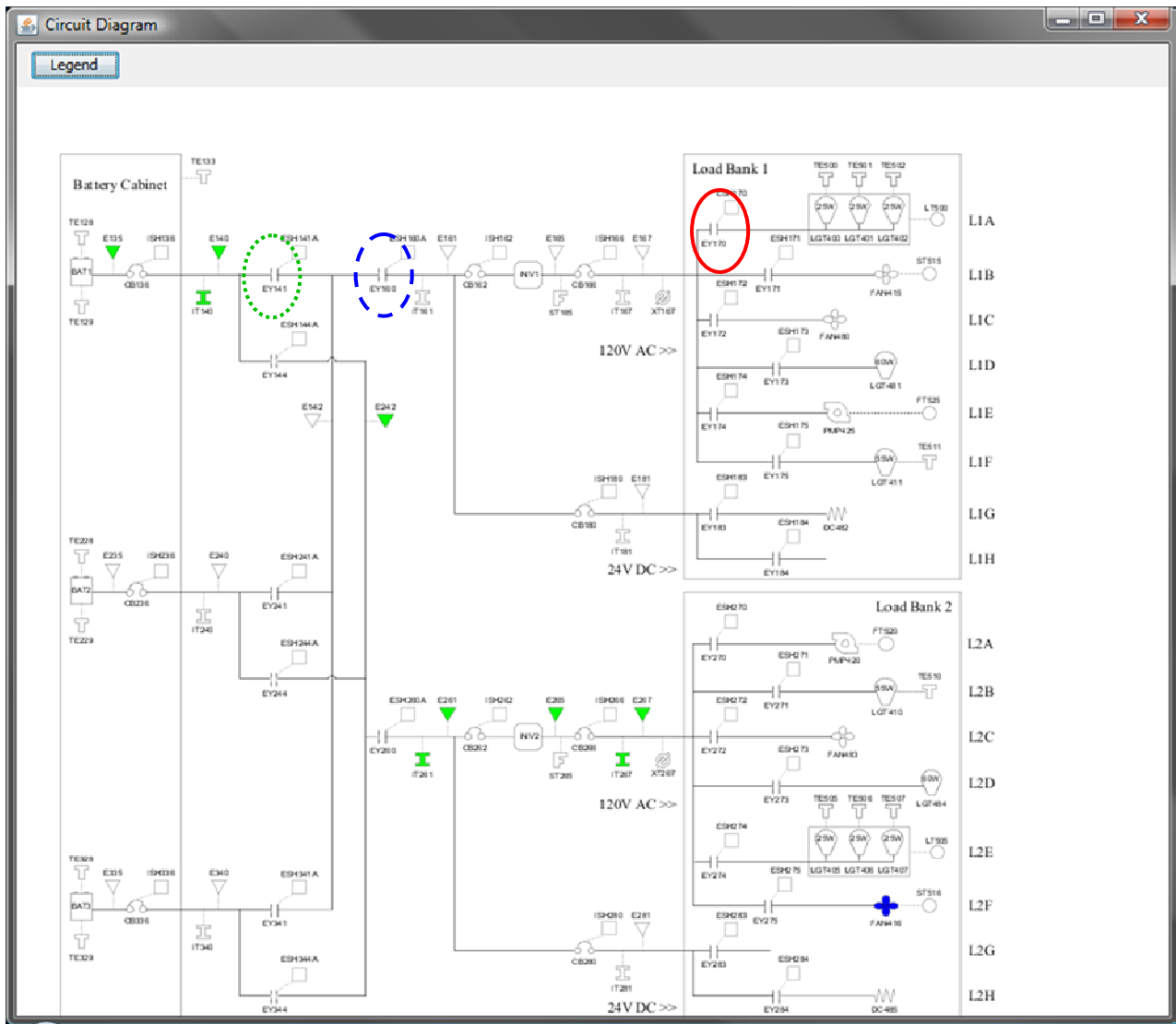
Figure 4 – Schematic of ADAPT System
