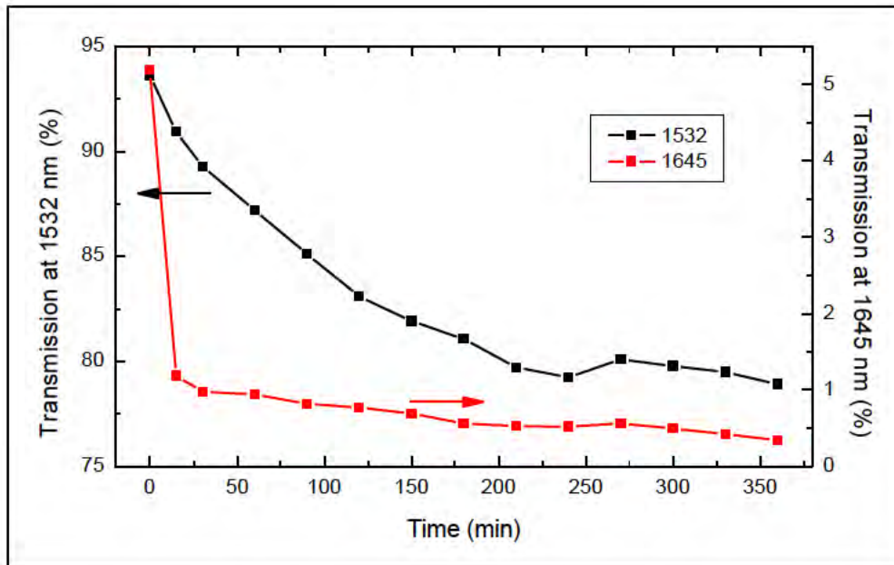
Figure 8. Transmission of HR-coated sample vs. bake time.
