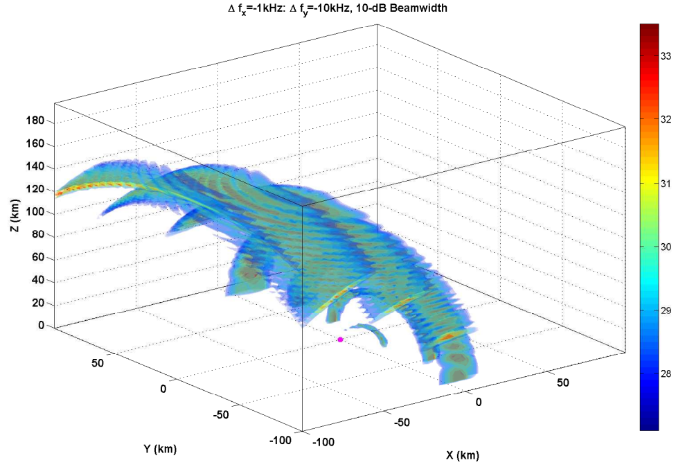
Figure 4.5: Transmit spatial pattern snapshot from a planar FDA radar for different frequency offsets. \Delta f_x = -1 kHz, \Delta f_y = -10 kHz
