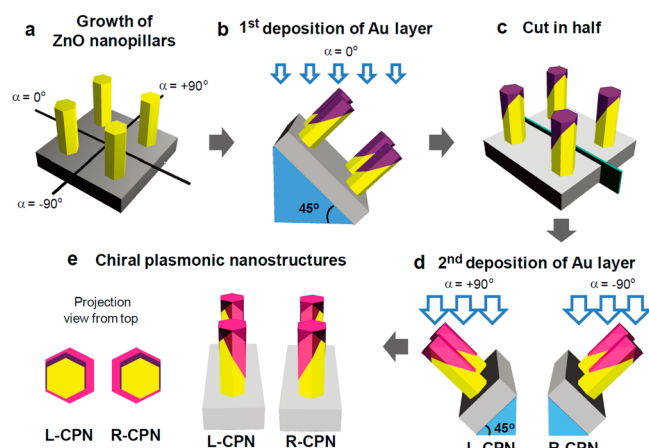
Figure 1. Schematics of the fabrication process. (a) ZnO nanopillars are grown onto substrate. (b) The first Au layer is deposited on top of ZnO nanopillar arrays from direction of \alpha = 0^\circ with an inclined angle of 45^\circ . (c) Samples are cut in half. (d) The second Au layer is deposited on each sample with different rotation. For the L-CPN sample, the direction of Au deposition is rotated to be incident from the direction of \alpha = +90^\circ . The other sample, R-CPN, is aligned to be exposed from \alpha = -90^\circ direction. (e) Asymmetric deposition of Au layers with inclined angle provides chiral nanostructures of Au-shell-coated ZnO nanopillars. A tilted view from \alpha = 180^\circ and the projection view from top are presented with schematics.
