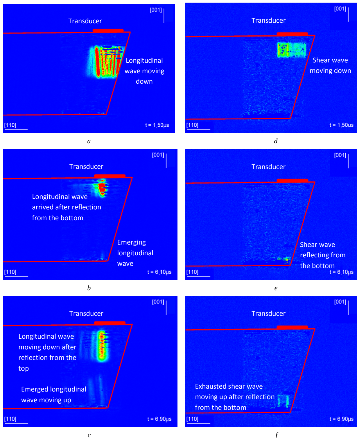
Fig. 8.4.5. Conversion of the SH wave into a longitudinal one on its normal reflection from the face (001) of the \text{TeO}_2 crystal. a, b, c – propagation, reflection and emergence of the longitudinal waves; d, e, f – propagation and reflection of the shear wave. Duration of the radiated pulses is 1\mu\text{s} , the carrier frequency is 27\text{ MHz} .
