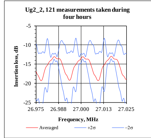
Fig. 6.2.4. Insertion losses of the sample Ug2_2 measured in a temperature uncontrollable environment. Thin blue lines determine a 95% confidence interval, \pm 2\sigma@27\text{ MHz}=2.35\text{ dB} .
