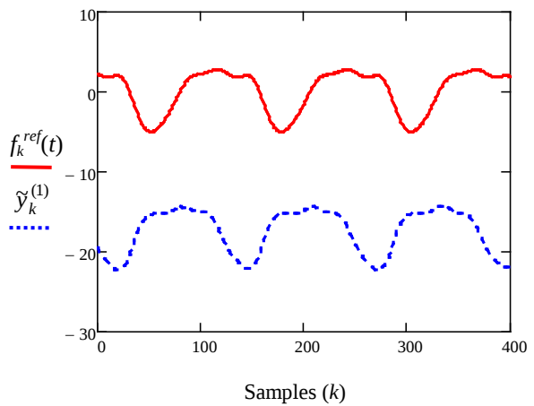
Fig. 10.3.5. Components of vectors \tilde{\mathbf{y}}^{(1)} and \mathbf{f}^{ref}(t) extracted from data obtained with sensor Ug2_2.
