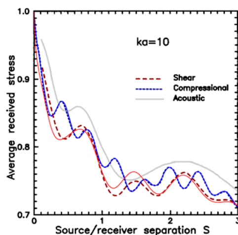
Fig. 9.4.4. Calculated diffraction losses for longitudinal and shear waves in an isotropic medium: comparison with [42]. The original black and white image was modified: dashed curves for shear and compressional waves were colored in red and blue; our data are presented by solid lines. An acoustic solution colored in gray is irrelevant to the task and was not analyzed.
