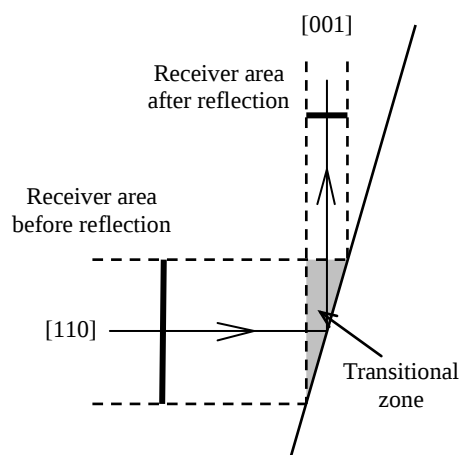
Fig. 9.4.5. The diffraction loss calculation geometry before and after reflection.
