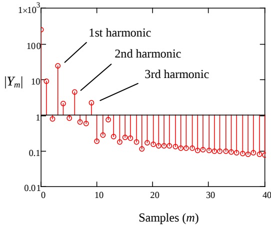
Fig. 10.3.2. Spectral components Y_m of vector \tilde{\mathbf{y}}^{(1)} extracted from data obtained with sensor Ug2.
