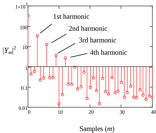
Fig. 10.3.4. Spectral components Y_m of vector \tilde{\mathbf{y}}^{(1)} extracted from data obtained with sensor Ug2_2.
