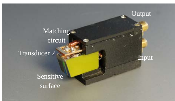
Fig. 2.3.3. The TIRUS sample Uj4 mounted into the “sensor housing”. The ( L \times H ) face of the crystal is coated with protective lacquer.
