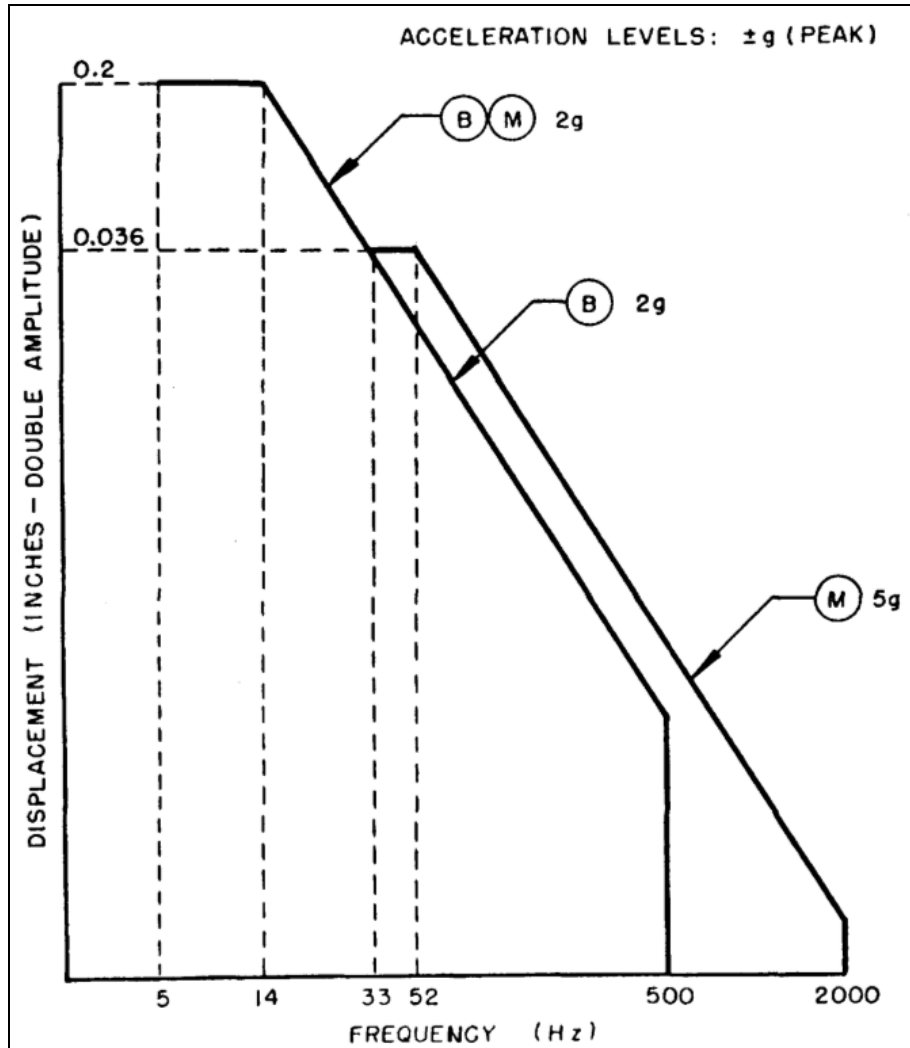
Figure 3-13. Vibration Test curves for Equipment Category C
