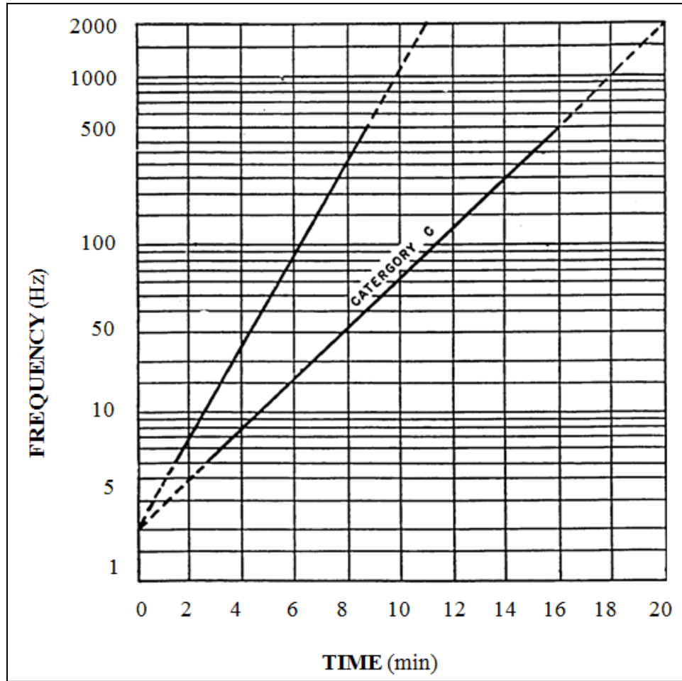
Figure 3-12. Logarithmic Sweep
