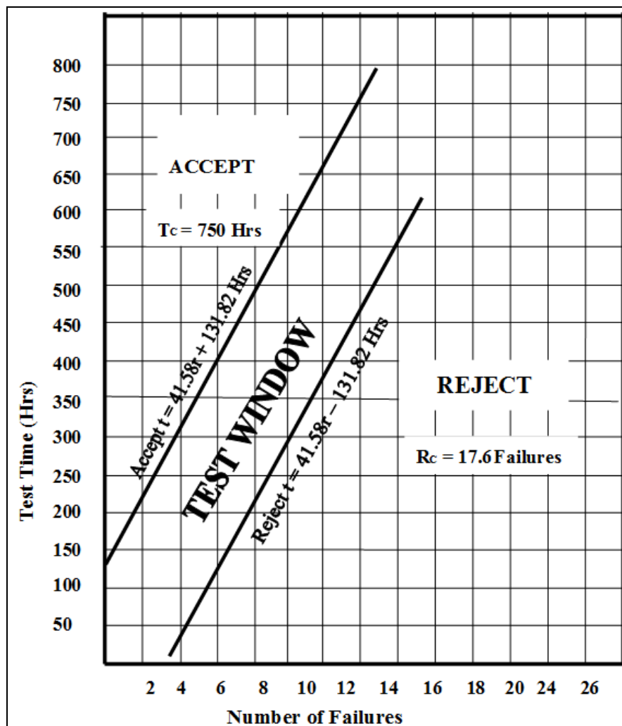
Figure 3-1. Reliability Test
