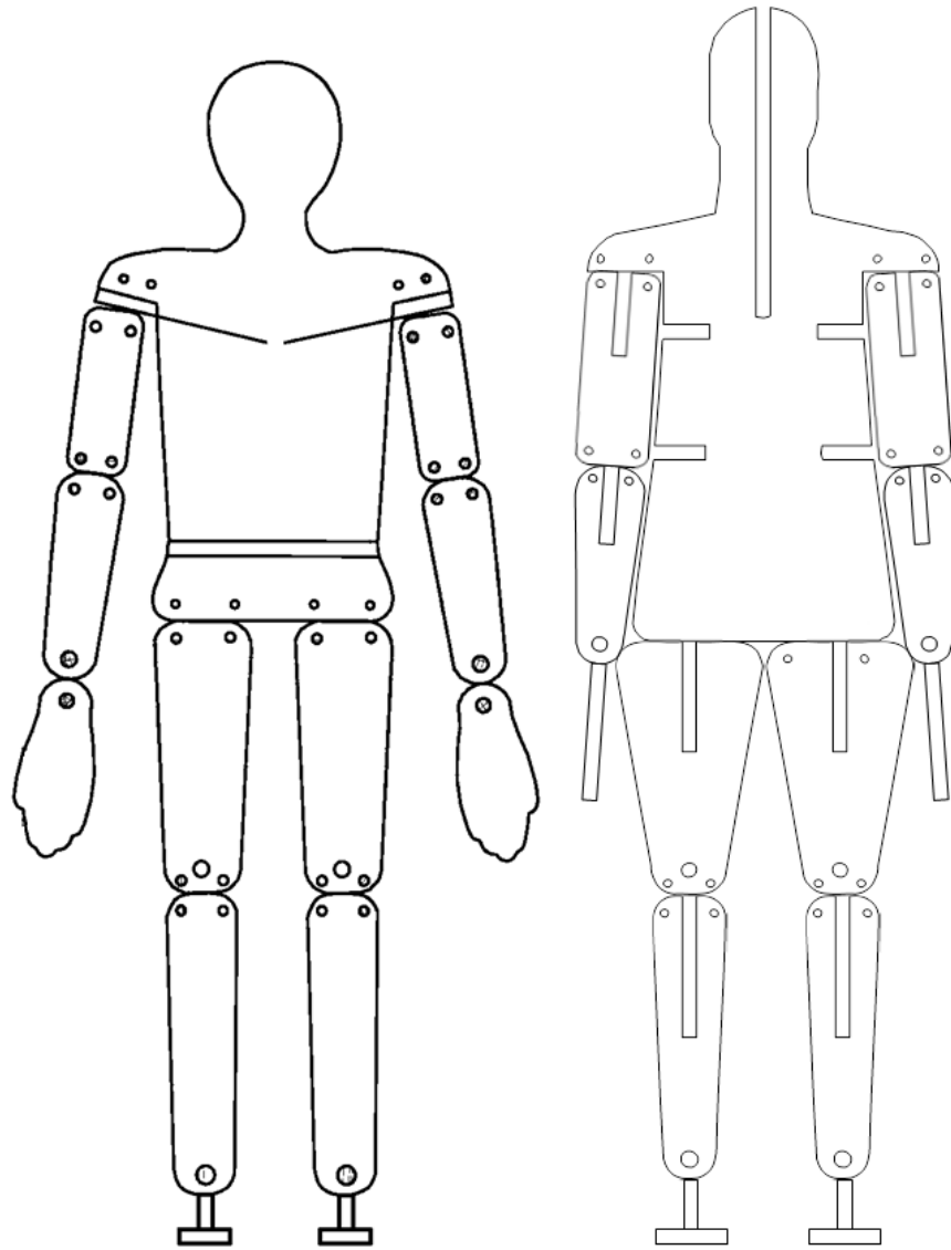
Fig. 5 The BRL (left) and the proposed ARL (right) plywood ballistic mannequins are side by side to show their components' respective sizes 49
