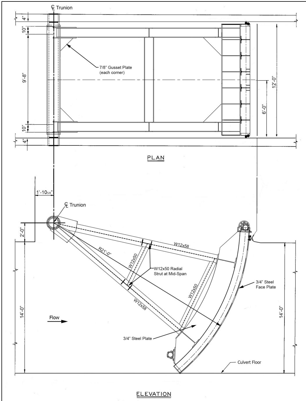
Figure 40. Plan and elevation of the Type 7 (recommended) valve.
