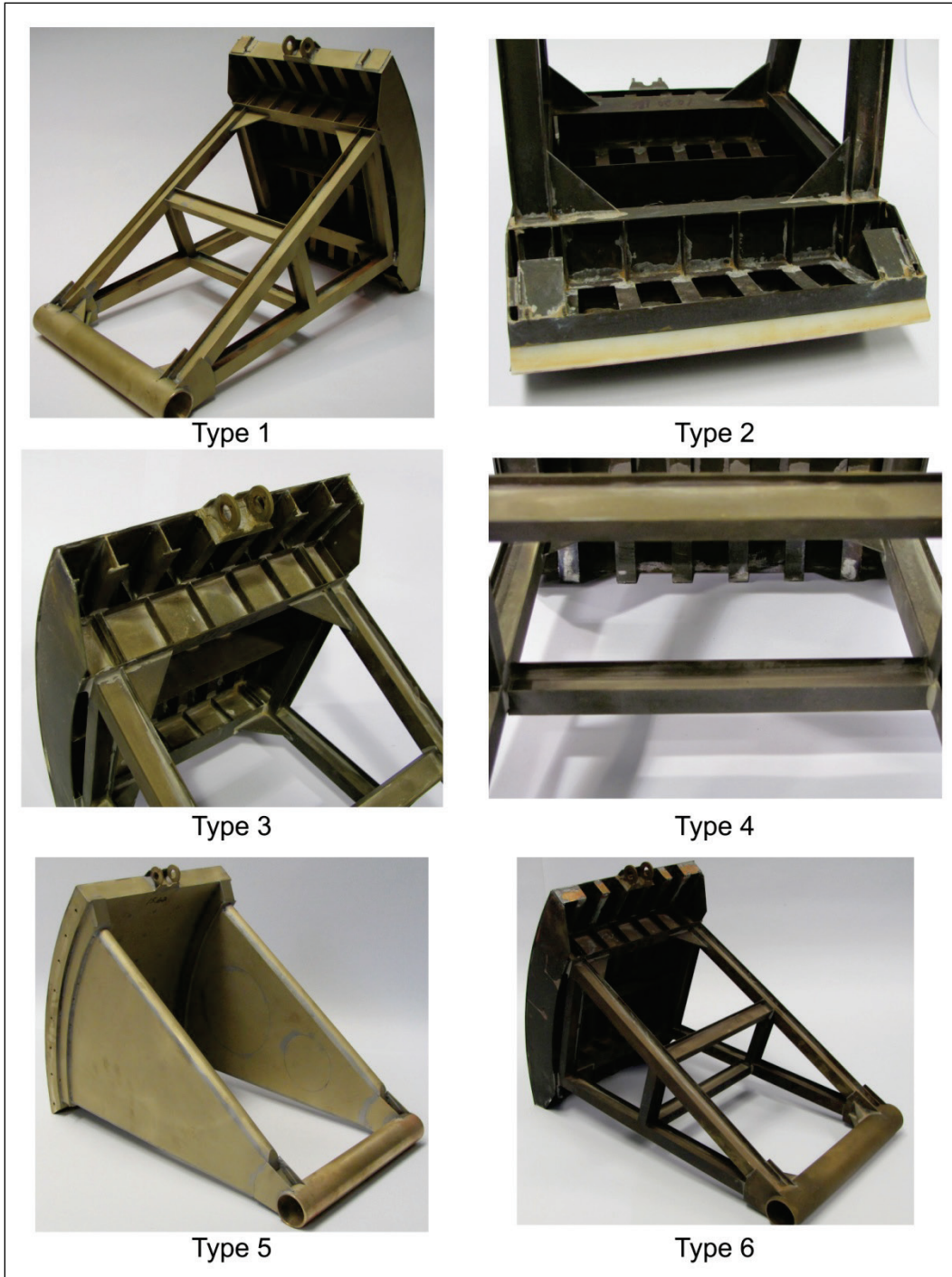
Figure 23. Types 1 (original), 2, 3, 4, 5 (double-skin-plate), and 6 valves.
