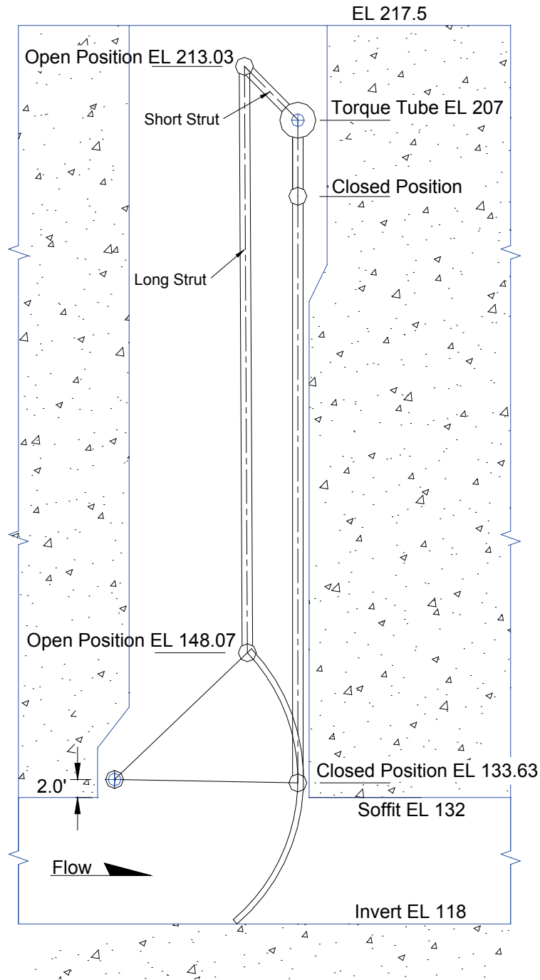
Figure 10. Valve machinery, Snell Lock filling valve.
