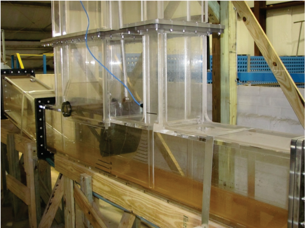
Figure 8. Dry bed view of the 1:15-scale model looking upstream.
