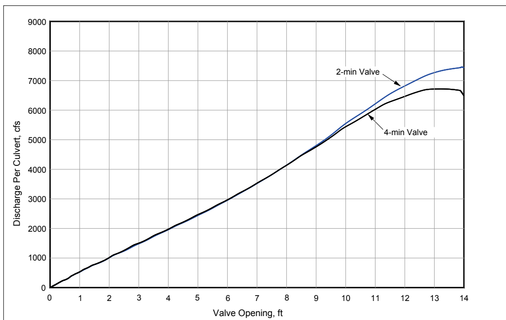
Figure 17. Discharge rating curves, 49 ft lift.
