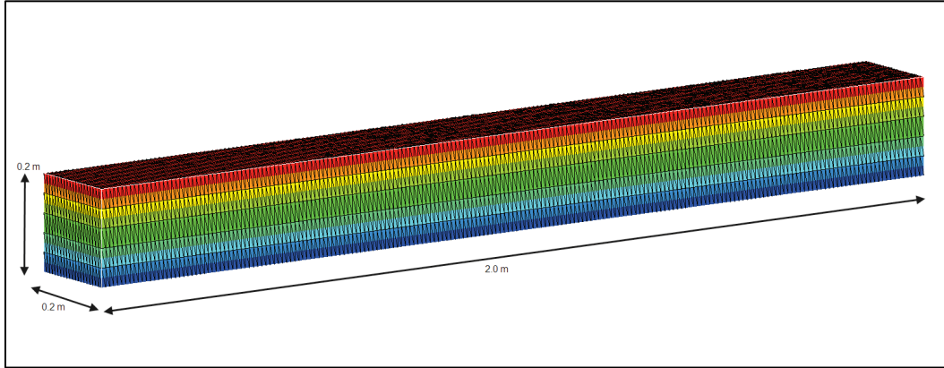
Figure 4. Domain for lock exchange.
