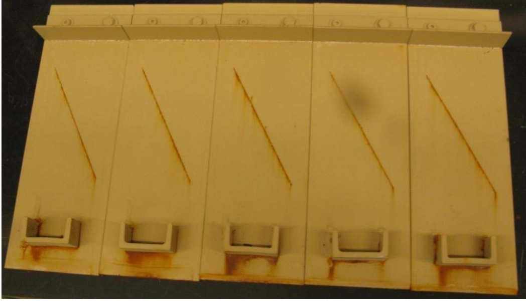
Fig. 32 Bonderite 7400 on multimetal panels primed with MIL-DTL-53030 after 80 cycles
