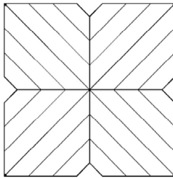
Figure 22. Solar cell front contact design of a highly transmissive butterfly pattern that avoids current crowding and applies the 30% Shockley-Queisser limit to the 1:6 electron-to-photon ratio. The resulting surface area covered by metal is 4.285%.
