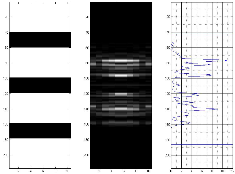
420 \mu m/820 \mu m Spacing, Full Bandwidth, Full Tilt, Low Resolution
