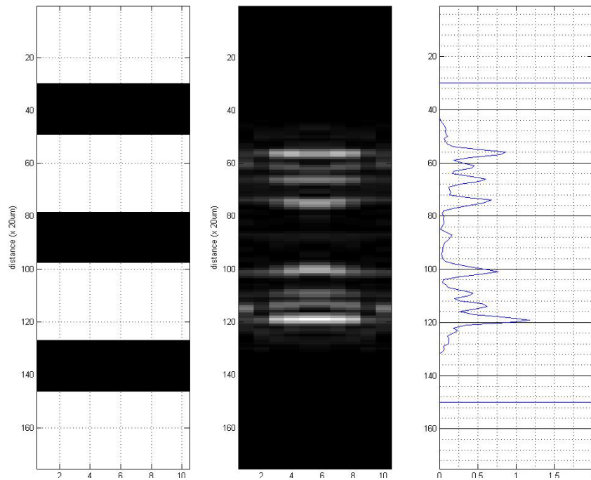
400 \mu m/600 \mu m Spacing, Full Bandwidth, Full Tilt, Low Resolution
