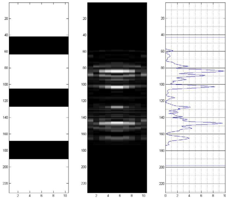
460 \mu\text{m} /860 \mu\text{m} Spacing, Full Bandwidth, Full Tilt, Low Resolution
