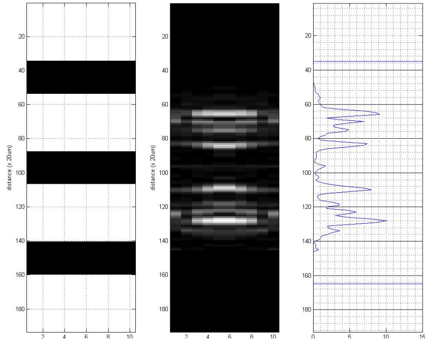
400 \mu\text{m} /700 \mu\text{m} Spacing, Full Bandwidth, Full Tilt, Low Resolution
