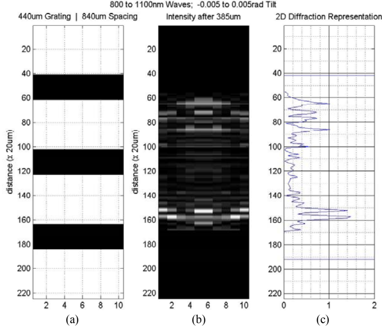
Figure 29. MATLAB® plots of (a) the 440/840μm grating matrix, (b) the interference pattern at 385μm, and (c) an intensity representation of the pattern. The simulated wavelengths were run in 10nm increments; the tilts were run in 0.001rad increments
