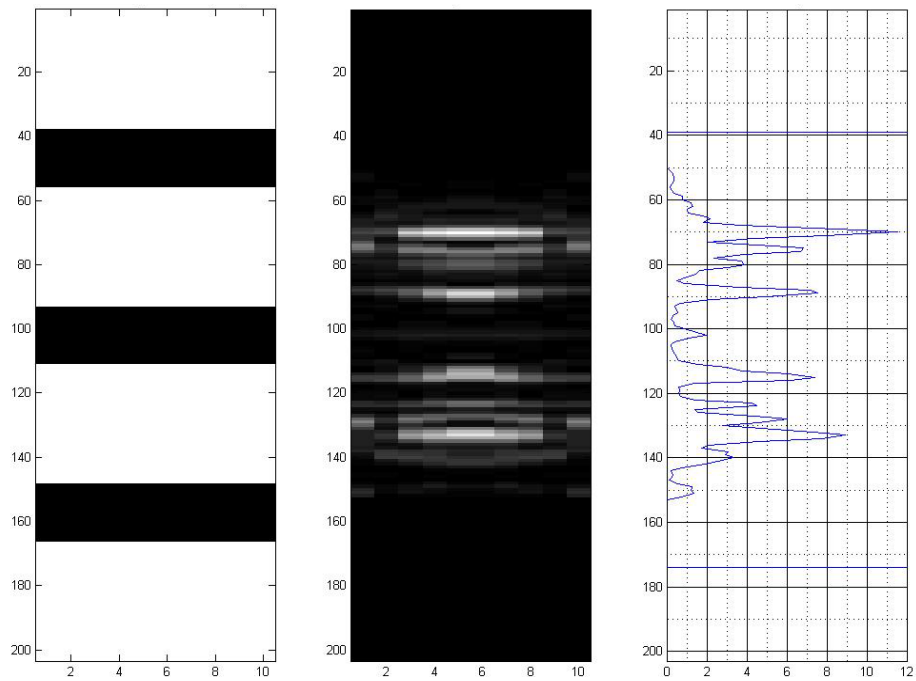
380 \mu m/780 \mu m Spacing, Full Bandwidth, Full Tilt, Low Resolution
