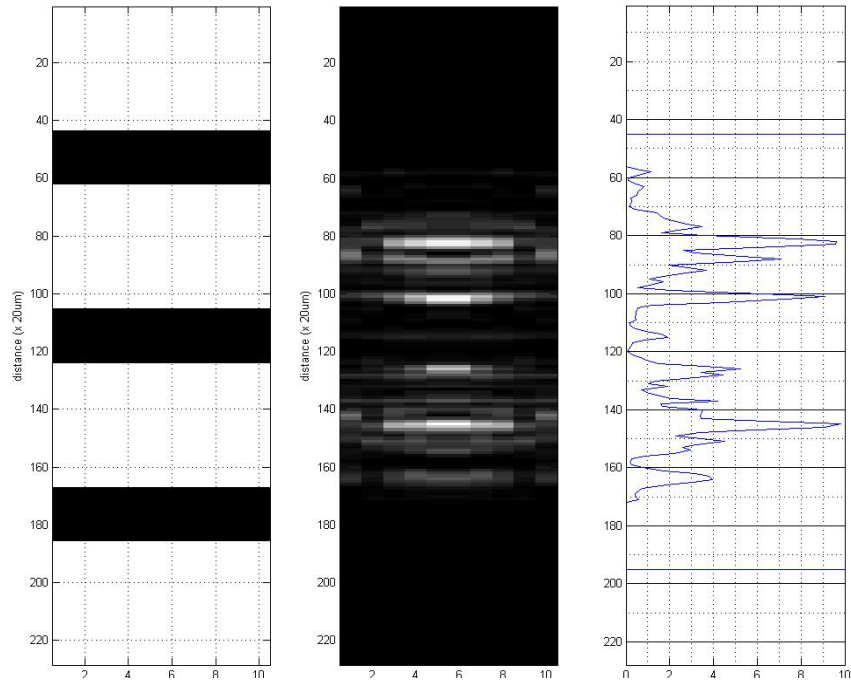
400 \mu\text{m} /900 \mu\text{m} Spacing, Full Bandwidth, Full Tilt, Low Resolution
