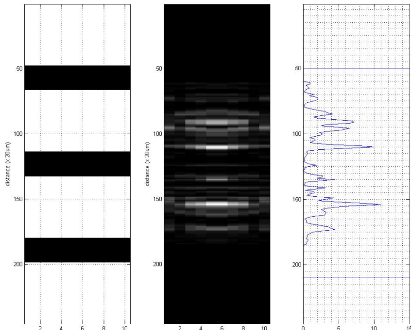
400 \mu\text{m} /1000 \mu\text{m} Spacing, Full Bandwidth, Full Tilt, Low Resolution
