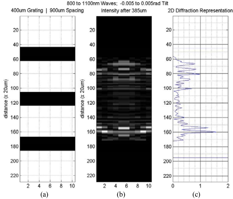
Figure 28. MATLAB ® plots of (a) the 400/900μm grating matrix, (b) the interference pattern at 385μm, and (c) an intensity representation of the pattern. The simulated wavelengths were run in 10nm increments; the tilts were run in 0.001rad increments.
