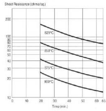
Sheet Resistance vs. Deposition Time
