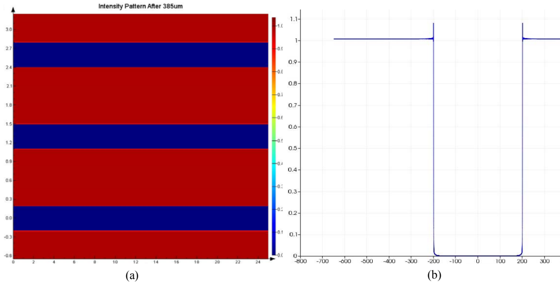
Figure 30. Lumerical® results showing (a) the far-field projection and (b) a single-period intensity plot and fringing effects from a plane wave propagated 385μm through the 400/900μm grating.
