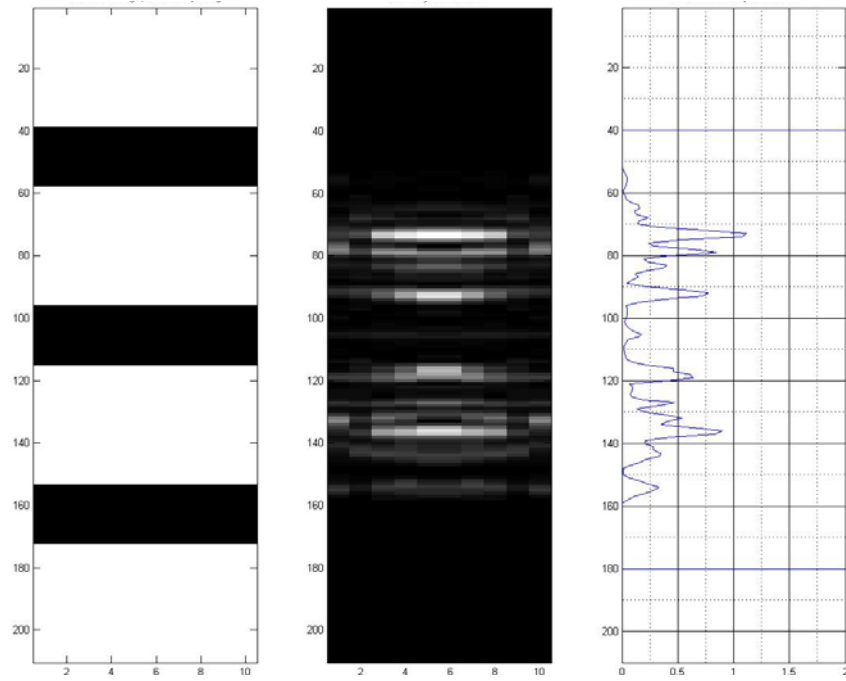
400 \mu\text{m} /800 \mu\text{m} Spacing, Full Bandwidth, Full Tilt, Low Resolution
