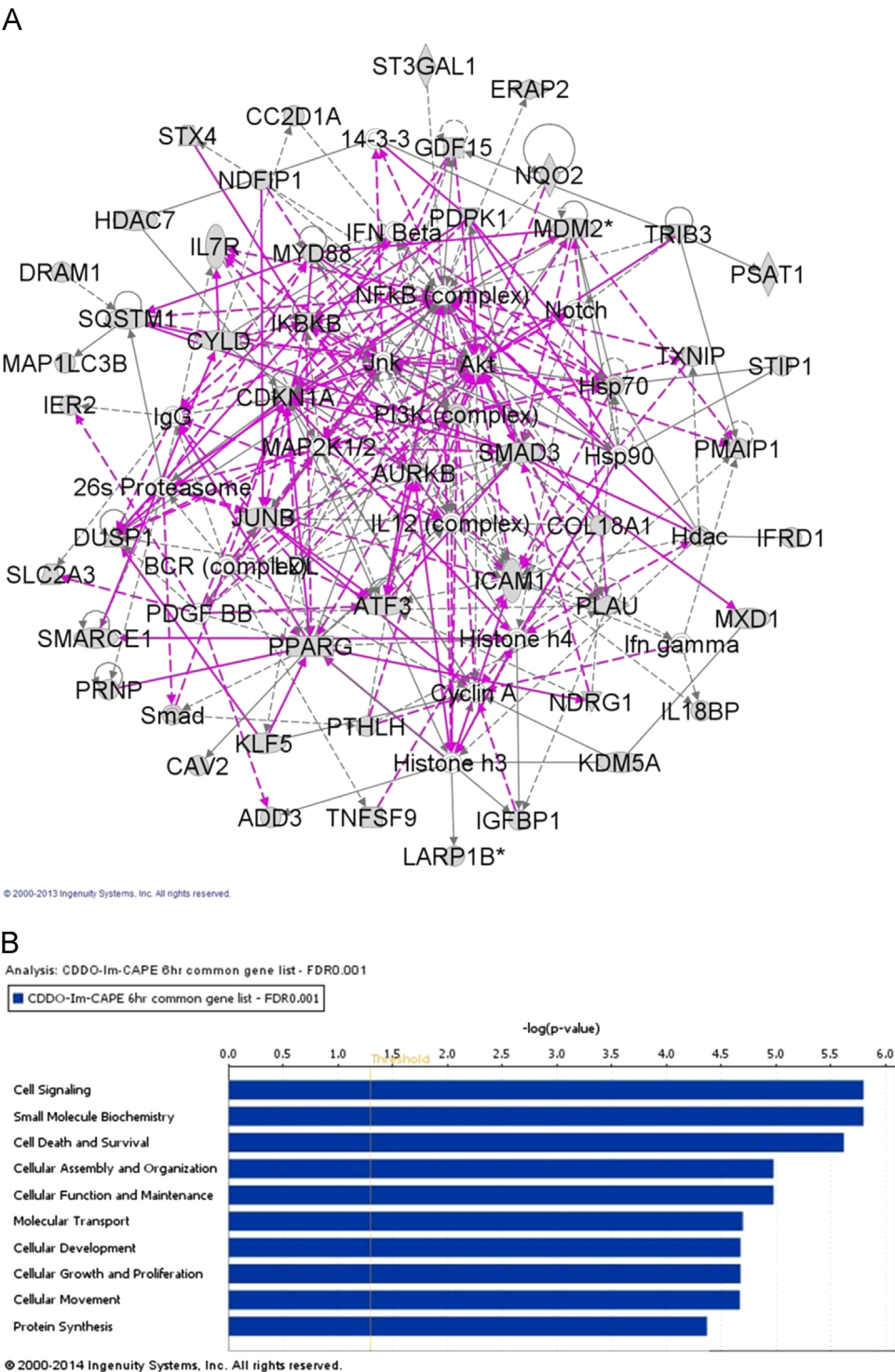
Fig. 4. Top scored network (A) and functions (B) of genes commonly altered by CDDO-Im and CAPE. Network associated functions involve cell death and survival, cellular development, and cellular growth and proliferation, which are among top 10 molecular and cellular functions commonly regulated by both compounds.
