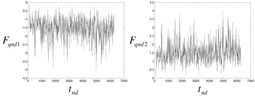
Figure 20. PV flux time series in the upper (left) and lower layers for r = 1 .
