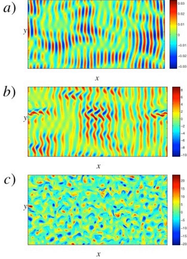
Figure 6. Snapshots of the PV anomaly field evolution in the large domain.
