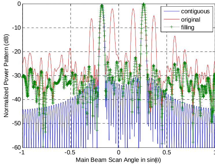
Figure 43. Pattern comparison of contiguous, original DDSA and virtual filled DDSA for 21^\circ fixed error and with 6 dB SNR at each element. Taylor amplitude taper ( \bar{n} = 5 , SLL = -30 dB) has been applied.
