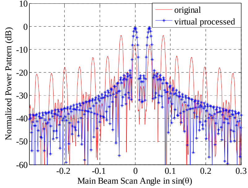
Figure 39. Comparison of original and synthesized antenna responses of 5 subarrays each with 30 elements, for signals (noiseless) incident from 0^\circ and 2.3^\circ .
