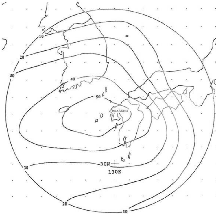
Figure 8. Mean Gust Radios (labelled as percentage) for Sasebo when a tropical cyclone of typhoon strength ( \geq 64 kt) is centered within 360 nm of the station. Locate the typhoon center by latitude and longitude and interpolate the ratio (percentage) value. Multiply the typhoon center wind speed by this percentage to get the wind speed value of the mean gust expected with the given center position and wind speed. Multiply the mean gust speed by 0.67 to find the mean one-minute average sustained wind speed.
