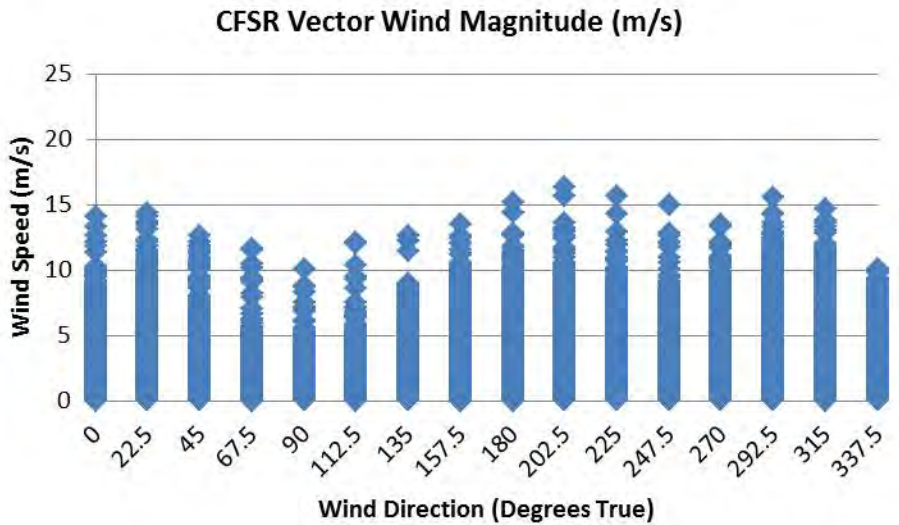
Figure 44. Wind speeds as a function of wind direction at CFSR gridpoint 33° N, 130° E for 2003 to 2010. Compare with Sasebo AMEDAS observations in Figure 16.
