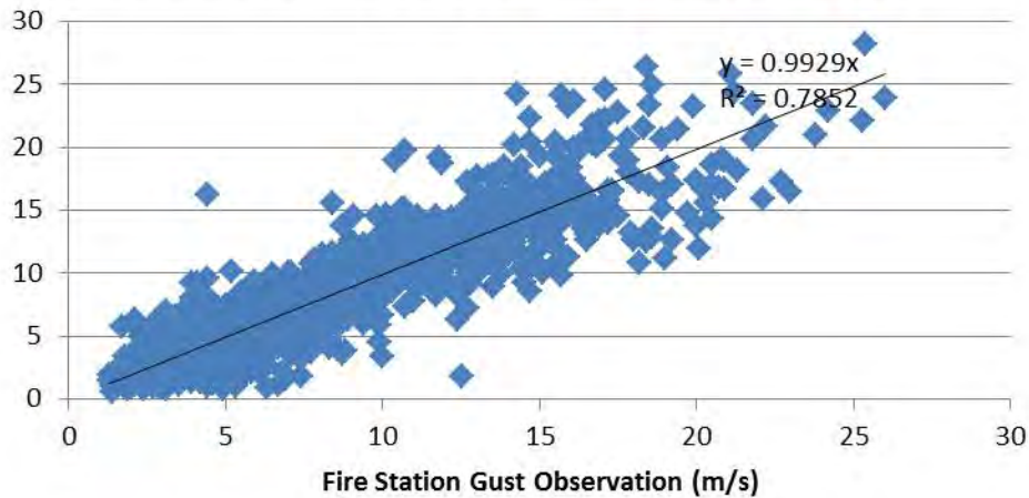
Figure 29. All available gust wind speeds at the Sasebo Fire Station vs. at the AMEDAS station. The regression equation is a linear fit with an imposed zero intercept. This is from the same set of observations in Figure 27.
