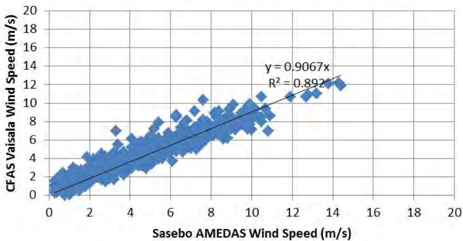
Figure 20. Depiction of all available simultaneous 10 minute average observed sustained wind speeds from Sasebo AMEDAS vs. CFAS Vaisala when AMEDAS 10 minute average direction was WNW. Displayed equation is a linear fit of AMEDAS to Vaisala wind speed with an imposed zero intercept.
