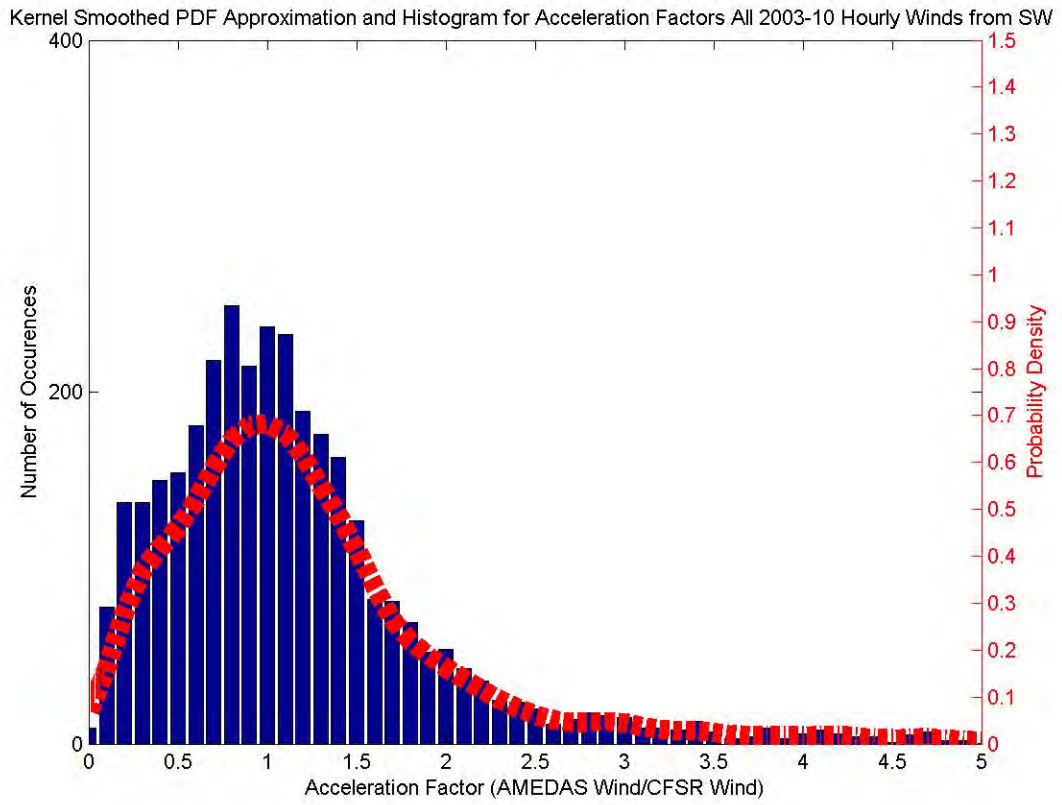
Figure 150. As in Figures 50 and 141, but for AMEDAS SW wind.
