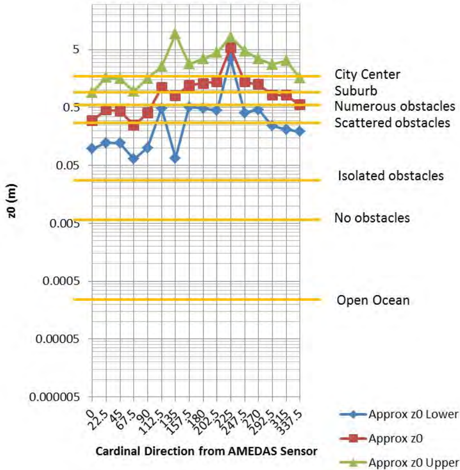
Figure 58. As in Figure 57, except for the PUW and AMEDAS observations for when TCs were within 200 n mi of Sasebo during 1990–1997 rather than 2003–2010.
