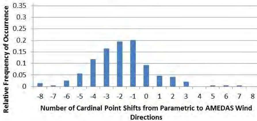
Figure 65. As in Figure 62, except for 194 observation times when TCs were within 200 n mi of Sasebo during 1998–2000, and thus were measured at the prior AMEDAS site.
