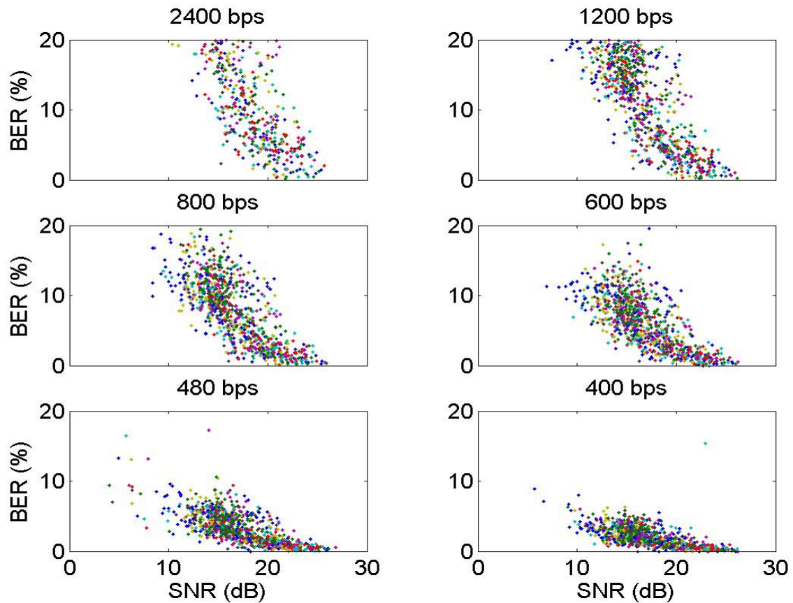
Figure 3: Bit-Error Rates as a function of SNR and data rate.
