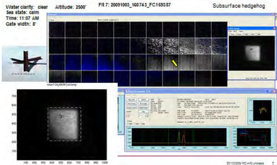
Figure 23. Hedgehog subsurface contact from BAE with algorithm results in lower left corner
