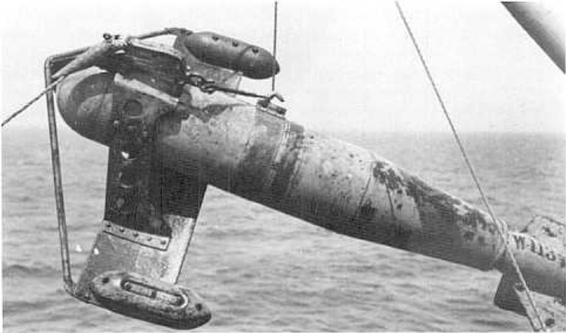
Figure 5. Paravane used by both the British and American navies during WWI (from Malia, 1991)
