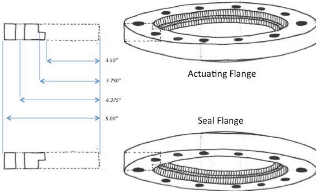
Figure 9. Seal and actuating-flange diagram.
