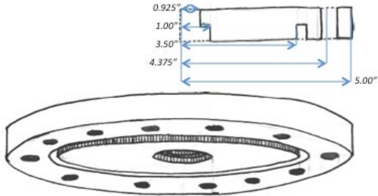
Figure 10. Actuating-plate diagram.
