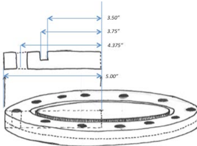
Figure 8. Seal-plate diagram.
