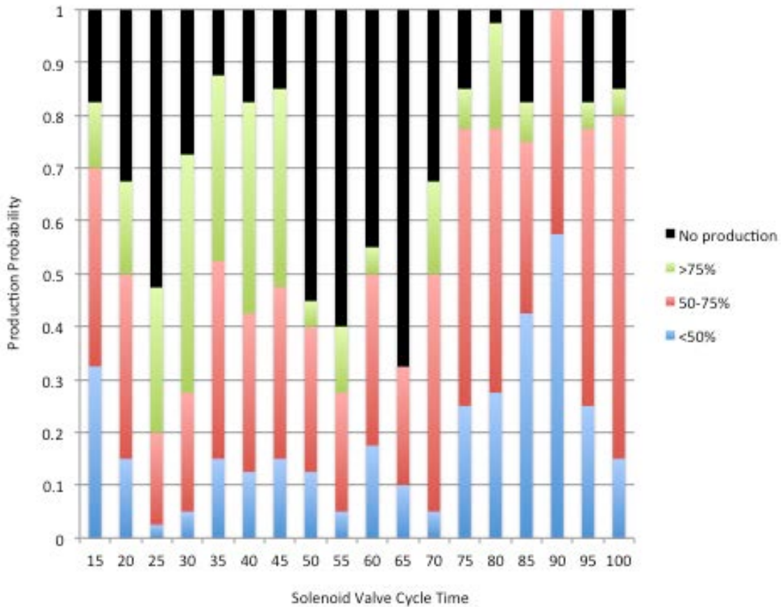
Figure 22. Bar graph illustrating the probability of production of vortex-ring bubble for a seal-pressure voltage of 1650mV and an actuation-pressure voltage of 2800mV. Each time increment consists of 40 individual actuation cycles. Black indicates that no bubble was produced. Blue indicates a bubble was produced, but dissipated before translating above the halfway point. Red indicates the bubble translated between half and three-quarters of the way up the water column. Green indicates the bubble translated greater than three-quarters of the way up the water column.
