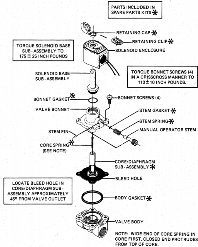
Figure 20. From ASCO form no. V5825R1, showing exploded diagram of 1/2 in. internally piloted, solenoid-operated diaphragm valve. Of particular interest is the core/diaphragm sub-assembly containing pilot orifice, bleed hole, and core spring.
