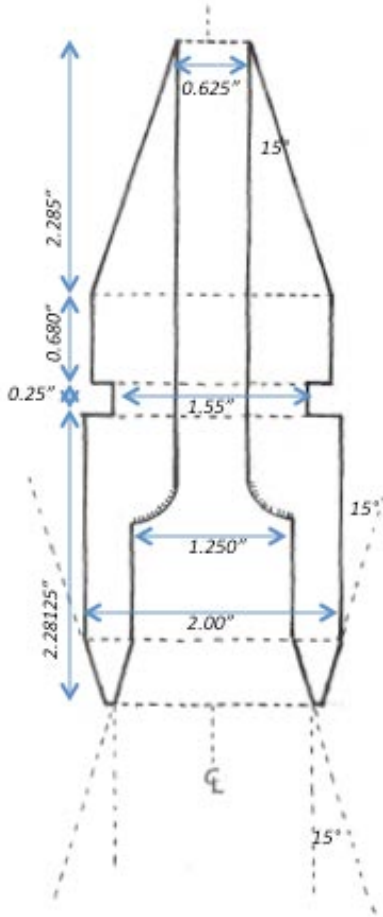
Figure 11. Final dimensions of nozzle based on characteristics described by Akhmetov and Shariff on the formation of vortex rings at a corner and the relationship between the angle of the nozzle and the expansion rate of the bubble radius
