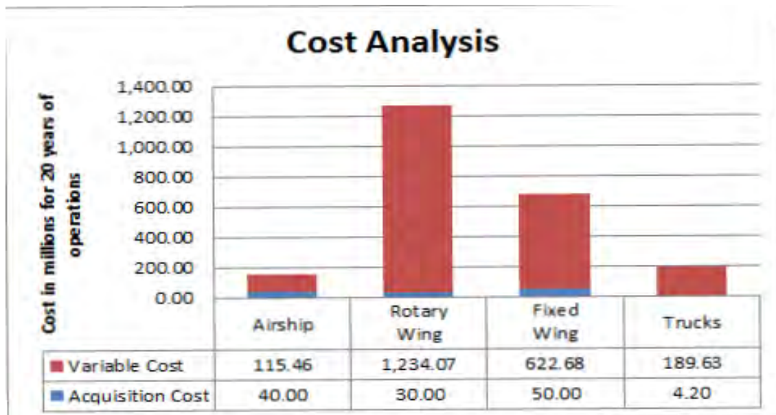
Figure 6.6: Total Cost of Operation for 20 Years of Operation by Vehicle Type
