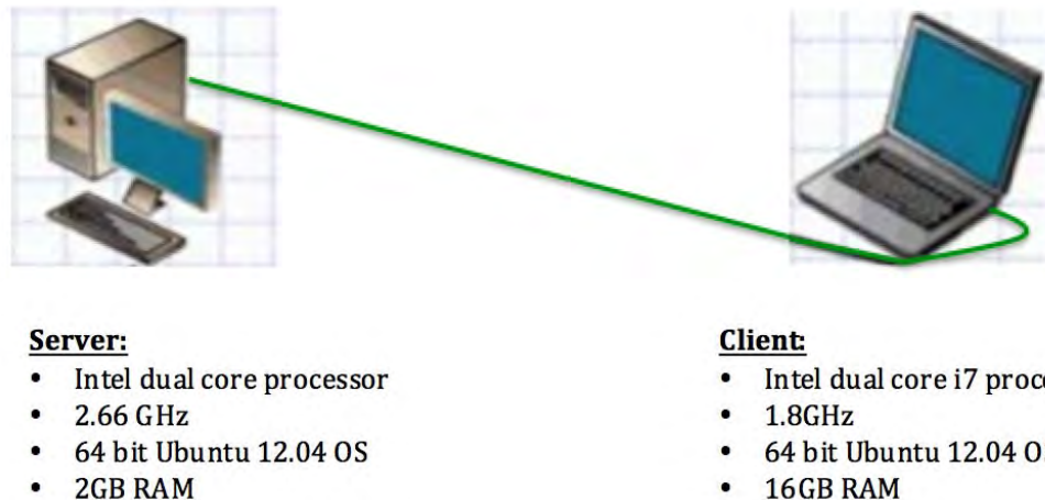
Figure 17. Testing Network Configuration
