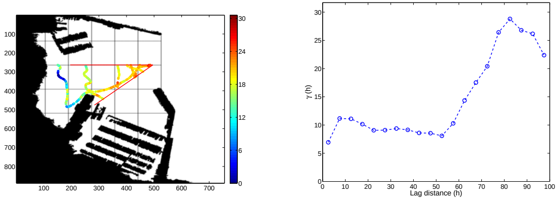
Figure 5.6: (Left) RSS measurements over a 45-degree bearing window. (Right) The resultant range semi-variogram. The maximum lag-distance for the semi-variogram is 100m. The nugget is approximately 6, the sill 26 and the range 80.
