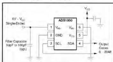
Figure 12. Measuring Single-Ended Inputs
