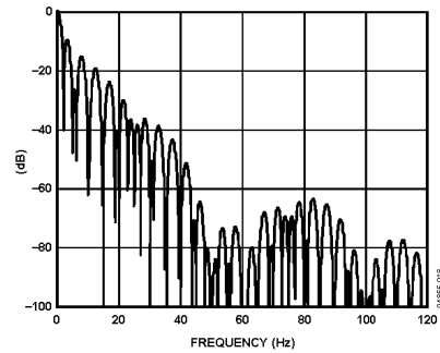
Figure 13. Filter Profile with Update Rate = 4.17 Hz
