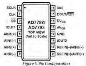
Figure 5. Pin Configuration
