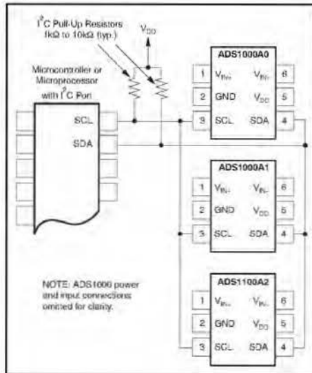
Figure 10. Connecting Multiple ADS1000s
