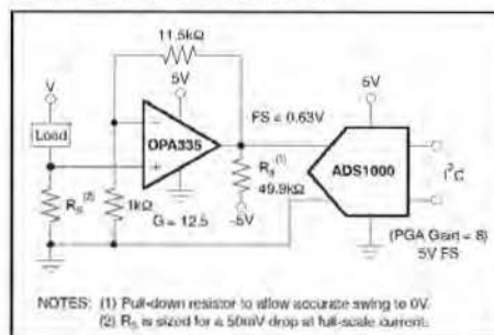
Figure 13. Low-Side Current Measurement
