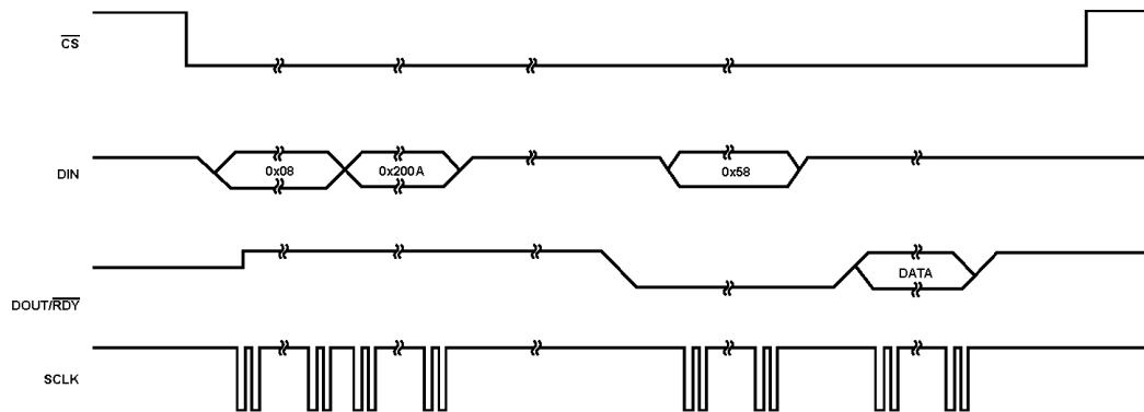
Figure 17. Single Conversion
