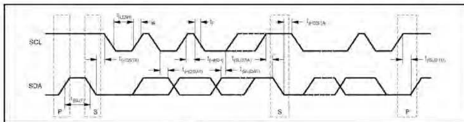
Figure 6. I²C Timing Diagram
