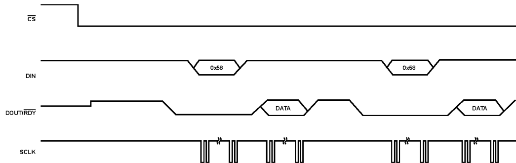
Figure 18. Continuous Conversion
