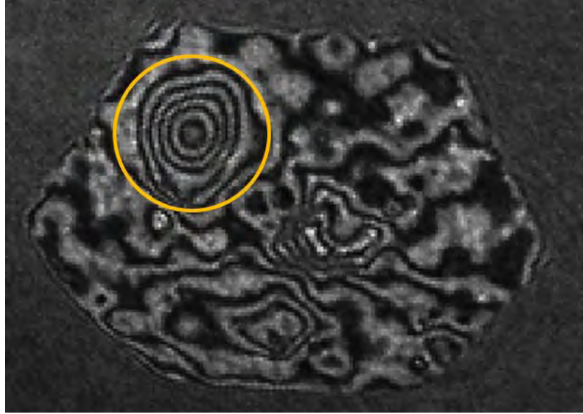
Figure 22. Interferometer image shows interference pattern when actuator is commanded.
