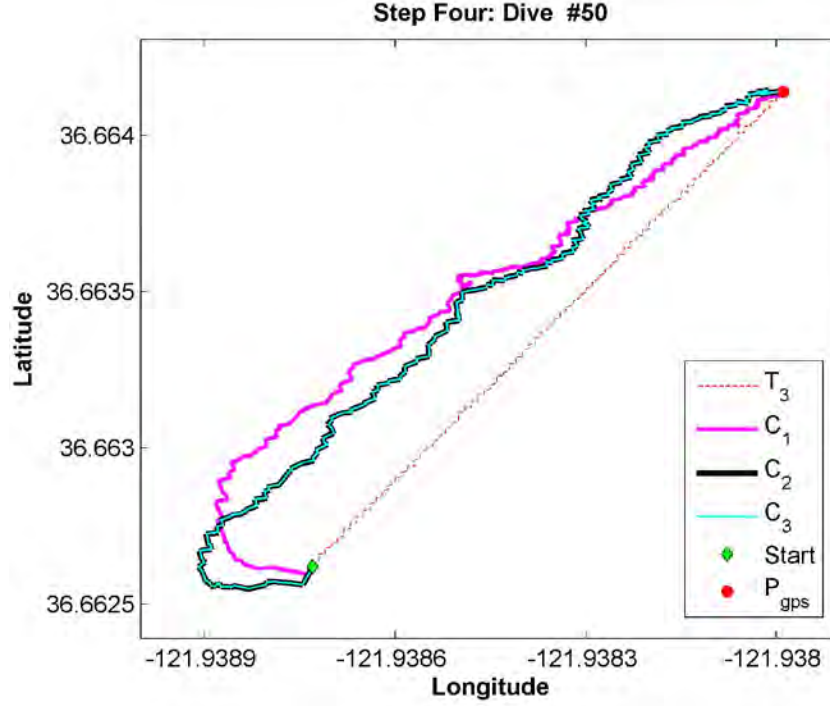
Figure 19. Downward Looking View of Three Types of Corrected Trajectory.
