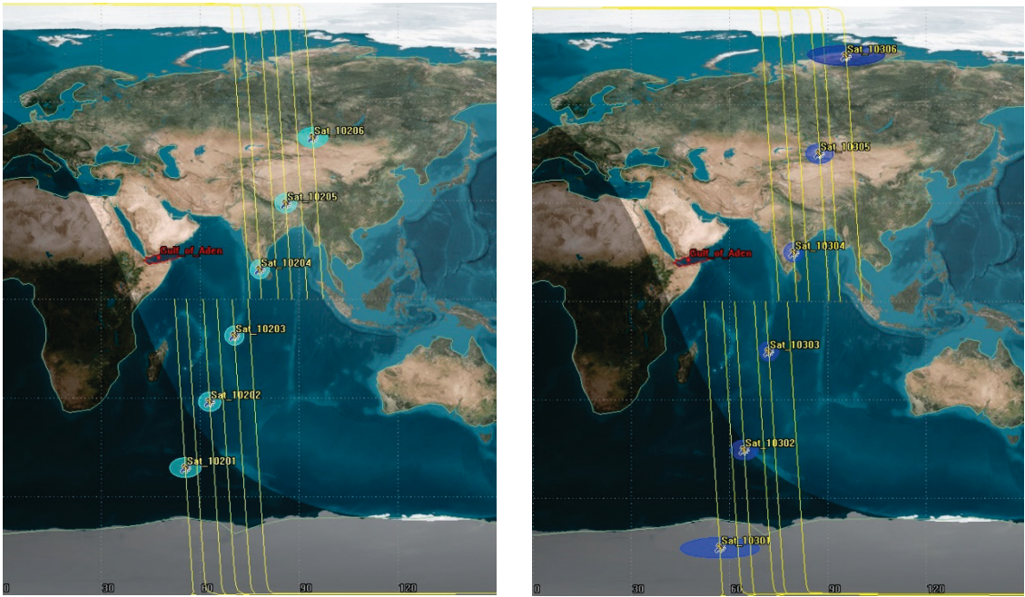
Figure 3. Comparison of ground tracks for nodal separations of 20° (left) and 30° (right).
