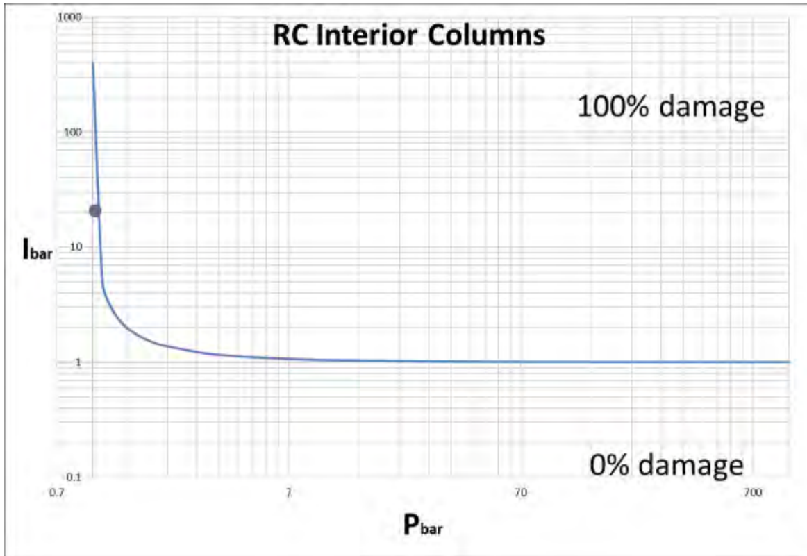
Figure 28. PI diagram of a Mark 84 detonating 27 ft away from a 12-in-by-12-in reinforced concrete interior column (After [2]).
