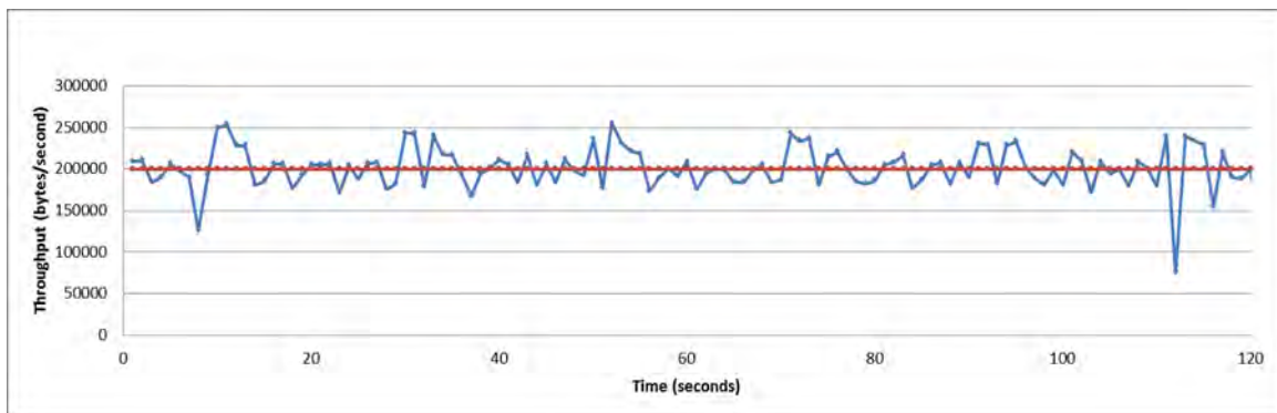
Figure 41. Throughput measured at Level 3 – one repeater at Level 2.5.
