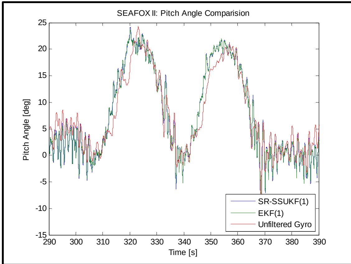
Figure 46. EKF(1) and SR-SSUKF(1) pitch estimates compared against an unfiltered gyro solution.
