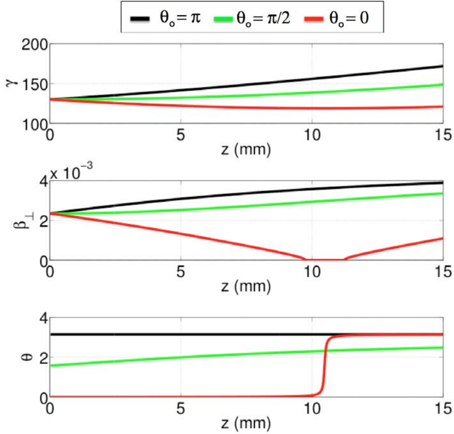
Figure 5.4: Simulation results for on-resonance but different initial \theta_0 for \gamma_0 = 130 , B_u = 45 . The top graph shows energy versus distance traveled for the first 15mm. The middle graph shows \beta_{\perp} versus distance. The bottom graph shows the evolution of \theta . The black curves shows \theta_0 = \pi . The green curves show \theta_0 = \pi/2 . Red curves show \theta_0 = 0 .
