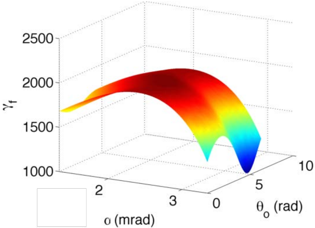
Figure 5.9: Surface graph of final electron energy \gamma_f versus initial \theta_o and \alpha for \gamma_o = 130 and B_u = 45 . There is a peak energy gain near \alpha_{\text{res}} \approx 2.4 mrad and \theta_o = \pi as expected.
