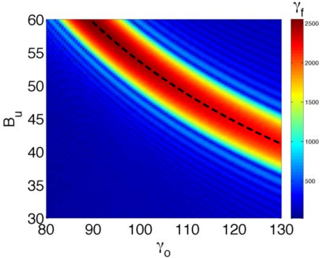
Figure 5.13: Simulation results showing an intensity plot of final electron energies with initial conditions that explore a range of external magnetic fields from B_{\perp} = 30 T to 60 T and \gamma_0 = 80 to 130. The dotted line indicates the \Delta\omega_{\text{O}\Lambda} = 0 contour.
