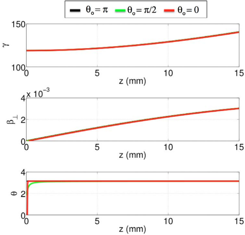
Figure 5.7: Simulation results for on-resonance but different initial \theta_0 for \gamma_0 = 119 , B_u = 45 . The top graph shows energy versus distance traveled for the first 15mm. The middle graph shows \beta_{\perp} versus distance. The bottom graph shows the evolution of \theta . The black curves shows \theta_0 = \pi . The green curves show \theta_0 = \pi/2 . Red curves show \theta_0 = 0 .
