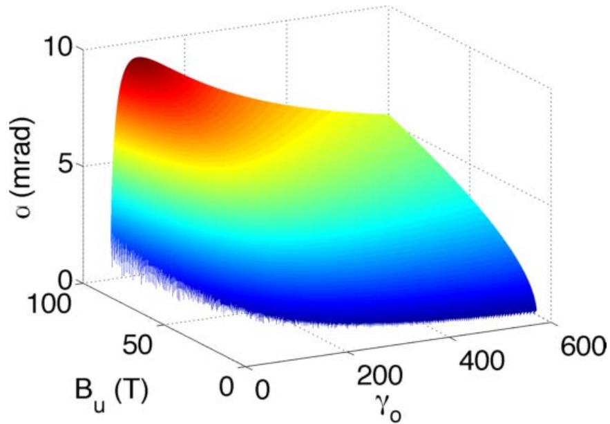
Figure 4.1: Shown is the the required injection angle for resonance as a function of initial electron energy, \gamma_0 , and external magnetic field, B_u , for a given \omega_r .
