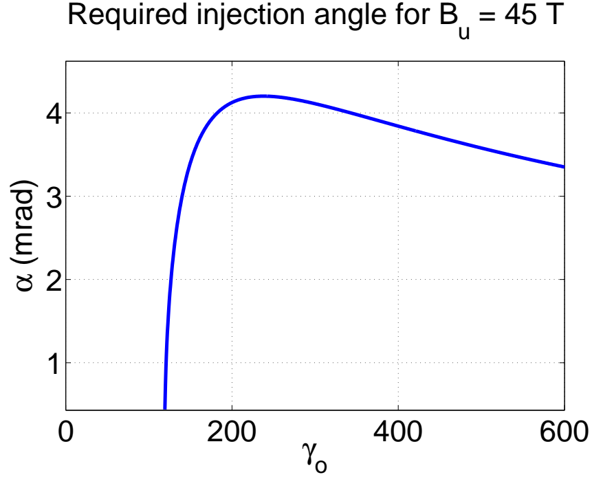
Figure 4.2: Shown is the allowed ordered pair combination of initial electron energy, \gamma_0 and initial injection angle, \alpha for a given magnetic field to guarantee resonance for a given \omega_r .
