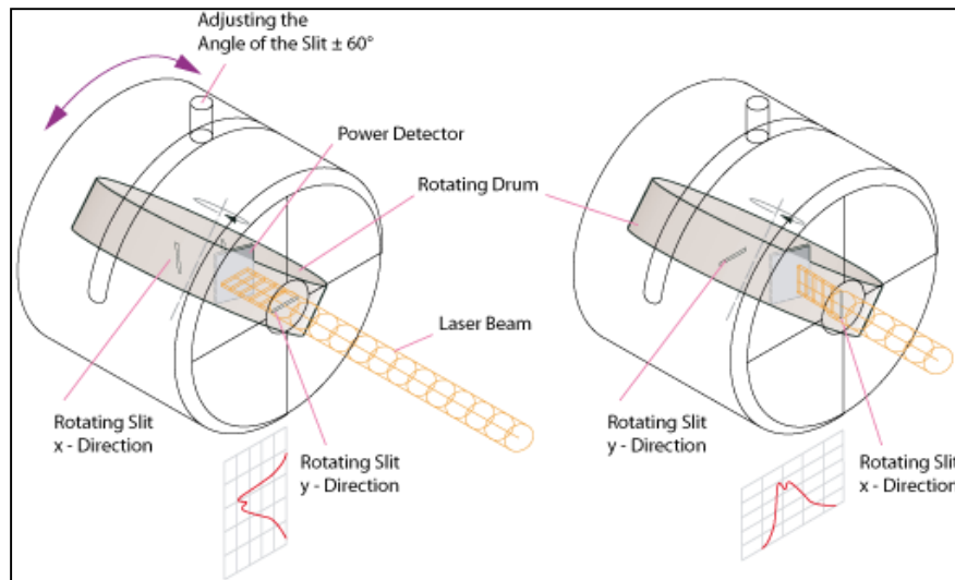
Figure 69. Scanning Aperture Technique Overview (From Thorlabs 2015)
