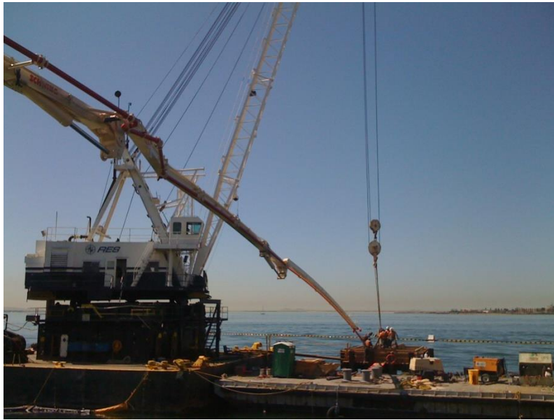
Figure 25. Pier External Support Resources (from R.E. Staite Engineering 2012)
