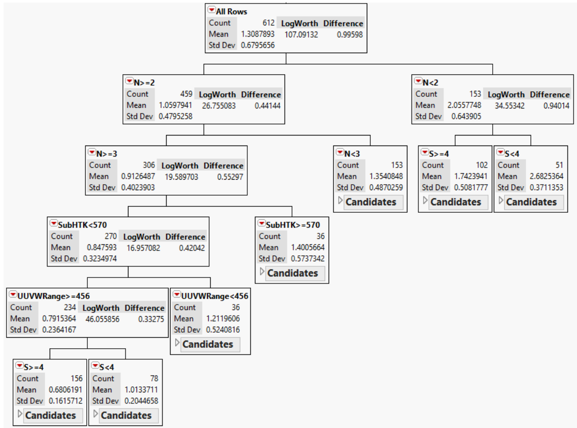
Figure 26. UUV data age MOE regression tree.
