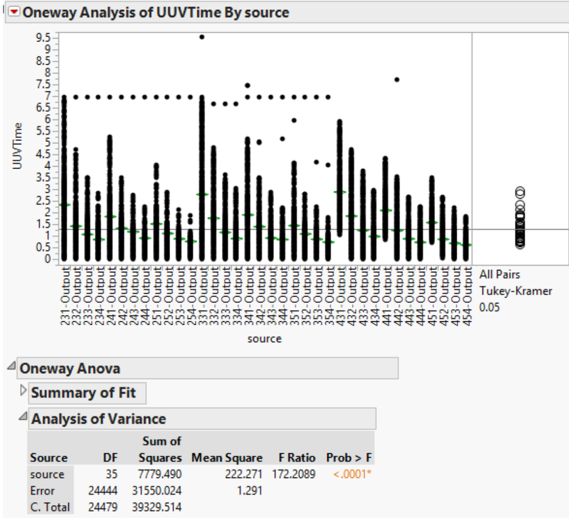
Figure 20. UVU data age ANOVA output.
