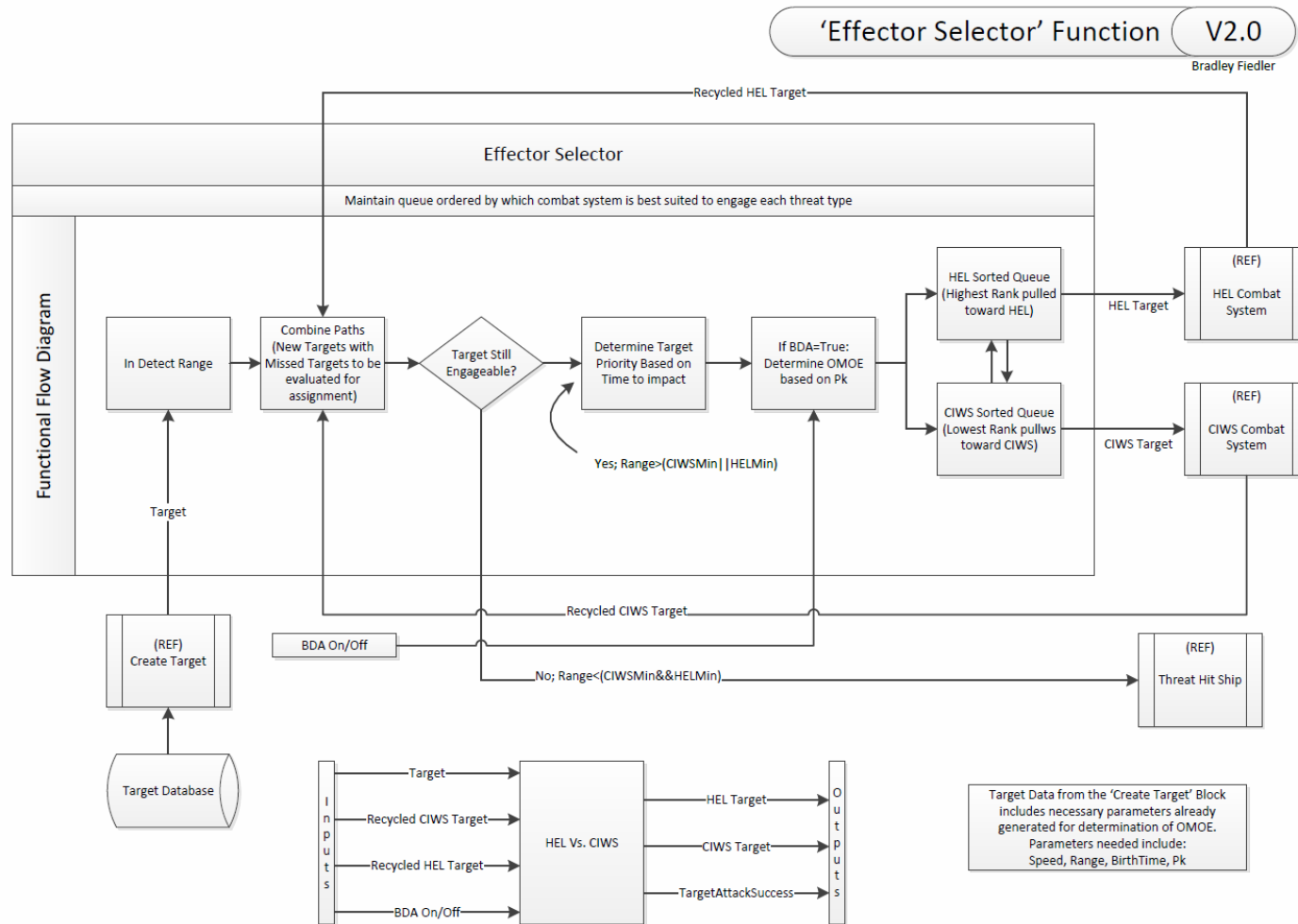
Figure 54. Weapon Selection FFBD
