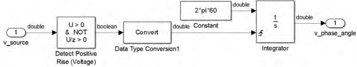
Figure 15. Simulink source voltage zero-crossing detection diagram.
