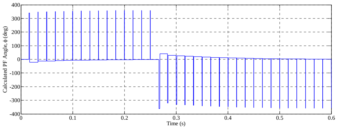
Figure 18. Power factor calculation with numerical integration error.
