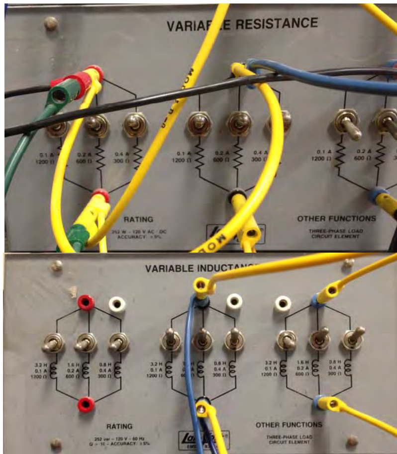
Figure 27. Variable load panels used in the experiment.
