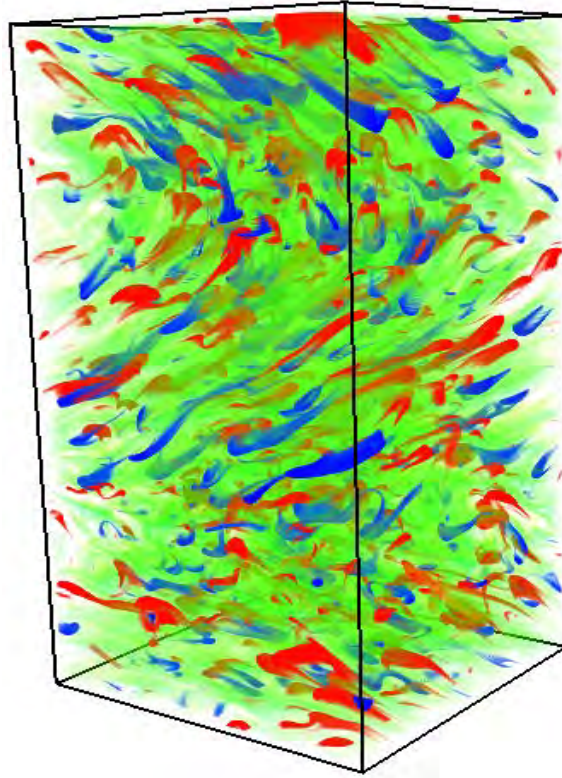
Figure 24. The simulation of version three shear model for R_i = 2 and a period of rotation of four hours. This showed the additional instabilities that contributed to the vertical transport of salt and heat.
