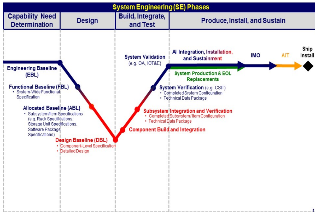
Figure 13. CANES Development Life Cycle (from PEO C4I 2009)
