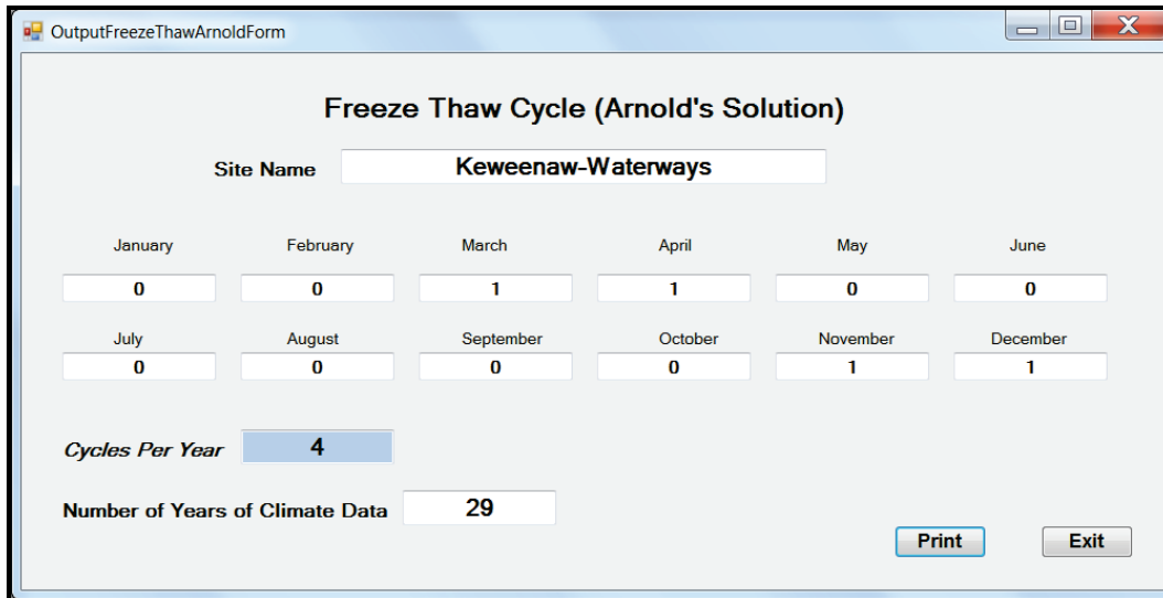
Figure 27. Example output for freeze-thaw intensity model for Keweenaw Waterways using Arnold's technique.
