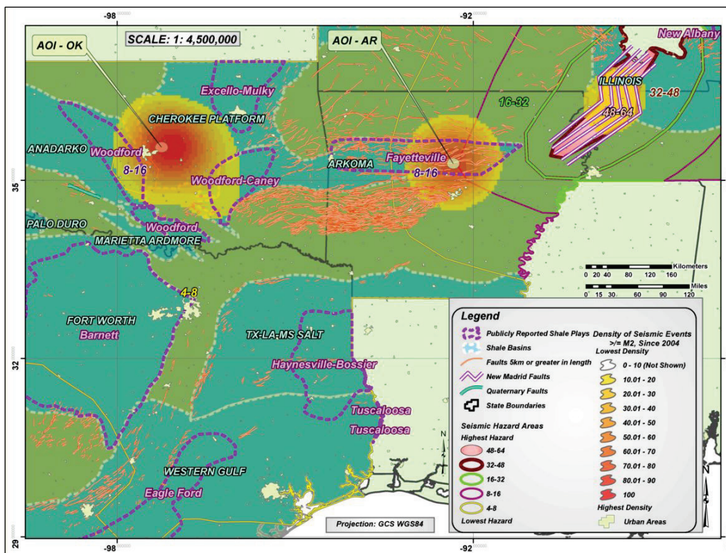
Figure 4. The seismic event density since 2004, for all seismic events M2.0 or greater throughout the study region focusing on Oklahoma and Arkansas (including the NMSZ), in relation to publicly reported effective shale plays and known faults in excess of 5 km in length. Callouts, AOI-OK and AOI-AR, indicate 112 km 2 areas of greatest event density (AOI-OK = 594 events; AOI-AR = 870 events).
