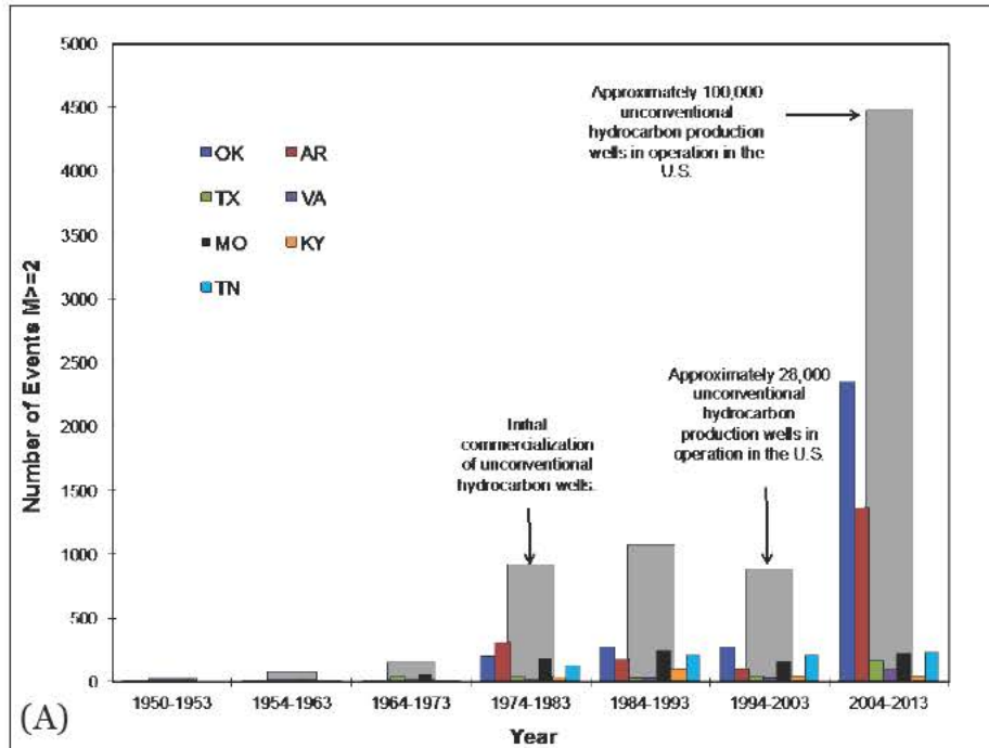
Figure 2. Distribution of seismic events per decade in the study region and the temporal increase in unconventional hydrocarbon production wells. Since 2004, there has been a significant increase in not only the number of events but also in the observed magnitudes compared to the previous three decades (A); Event distributions of the past three decades indicating regional completeness at M2.0 and greater post-1974 (B).
