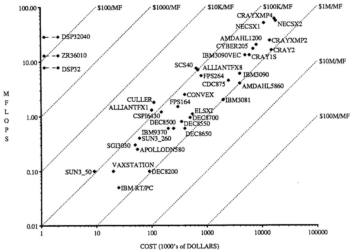
Figure 2-4. Computer System Cost Performance.
