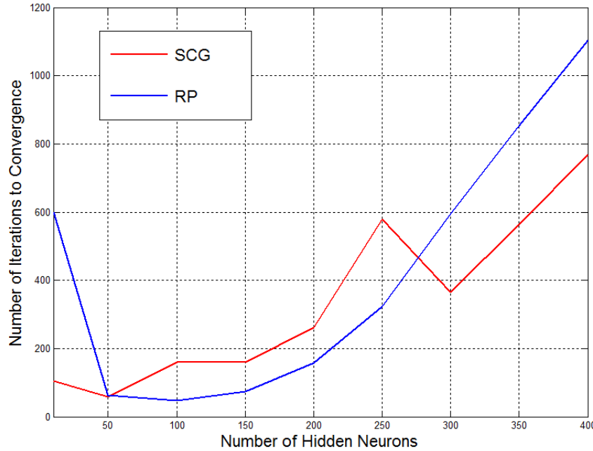
Figure 30. The number of iterations to converge to \varepsilon for each topology and learning algorithm combination during the training phase. Hough transformation features are used for training a multi-class classification neural network. As the size of the hidden layer increases, the number of iterations to convergence increases.
