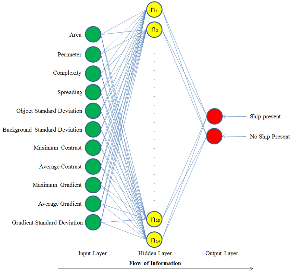
Figure 15. A neural network is designed for binary classification using geometric and photometric features for training. The eleven features are the inputs, with a variable hidden layer size, and two output neurons for a positive or negative response for a ship present in the image.
