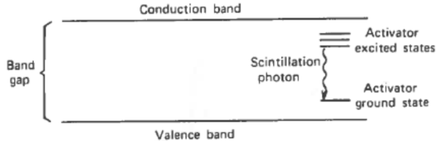
Figure 8. Energy band structure of an activated crystalline scintillator, from [5, p. 232].
