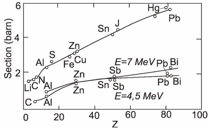
Figure 3. Inelastic scattering cross section (lower curves) of target nuclei with atomic number ( Z ) for the neutron energies 4.5 MeV and 7 MeV. Total interaction cross section values are given by the upper curve, from [12].
