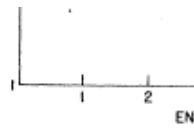
Figure 1. Experimentally determined energy spectrum of Cf-252 fission neutrons, from [8].
