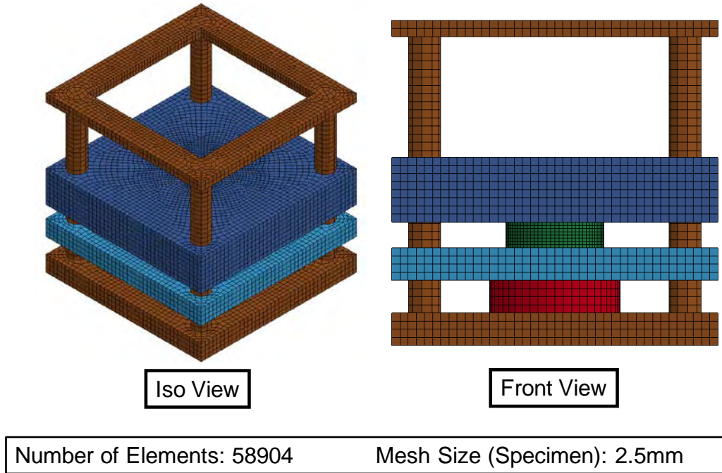
Fig. 5 FE model of the component loading test
