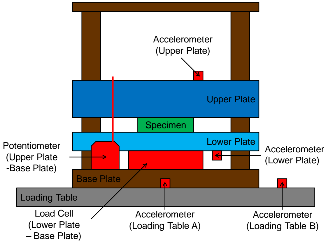
Fig. 4 Arrangements of sensors in the test setup
