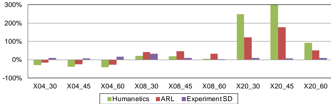
Fig. 27 Encircled area errors of FEAs versus experimental data. (LSTC model's errors are omitted due to poor differentiation in the loading-unloading curves.)
