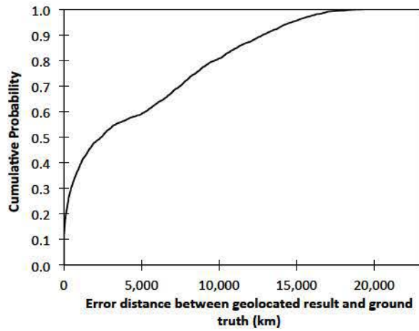
Figure 4.1: CDF for error distances of 4,152 targets from six vantage points.
